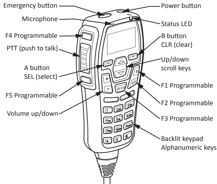
Figure 4 - Controller Microphone
