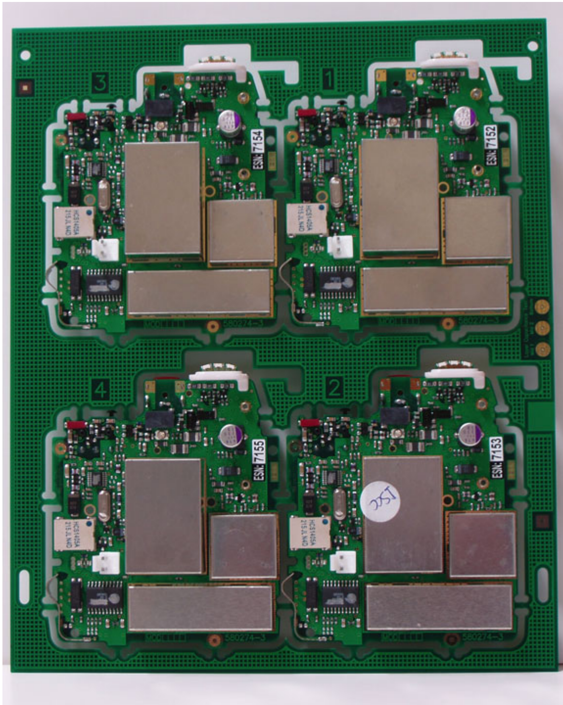
Figure 3 - PCB, top view (panel of 4 in biscuit)
