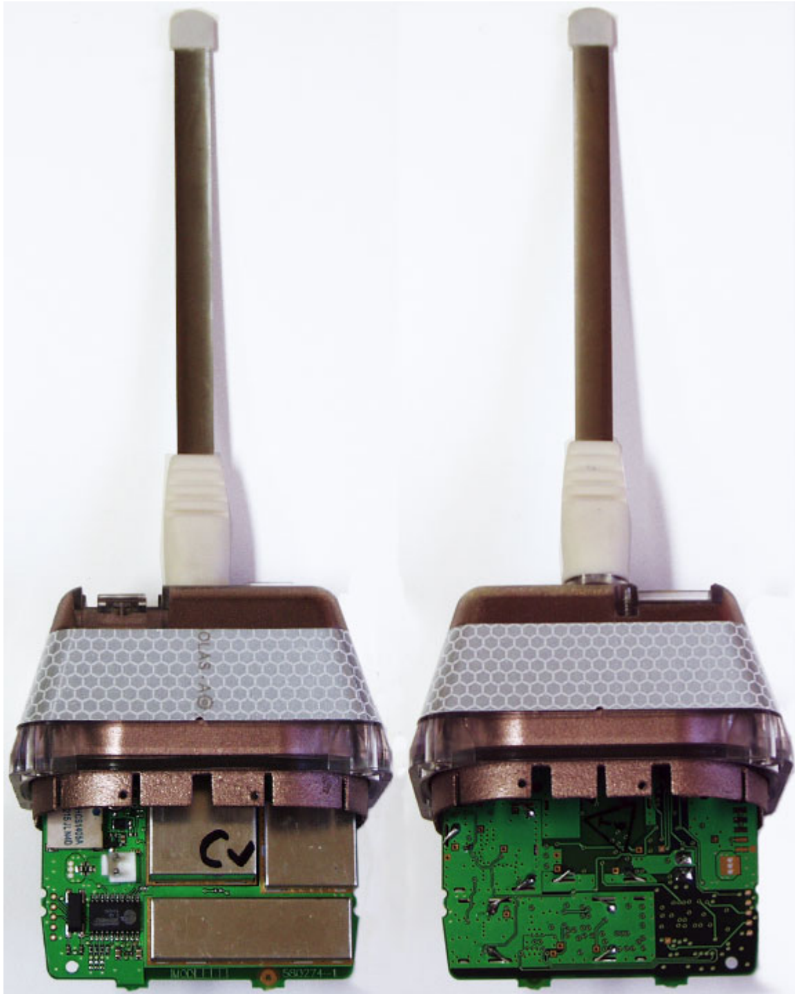
Figure 2 - Cap assembly view (front & rear)
