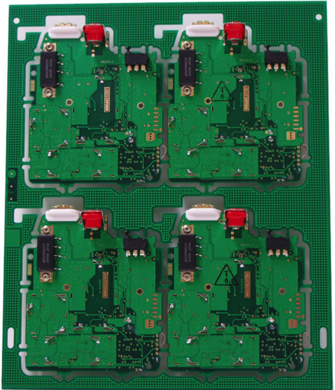
Figure 4 - PCB bottom view (panel of 4 in biscuit)
