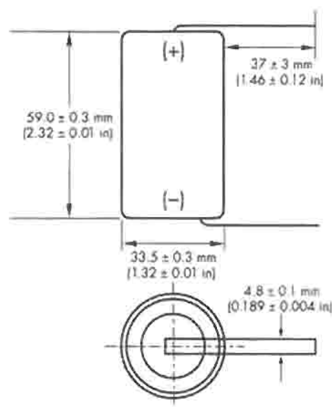
overall dimensions
