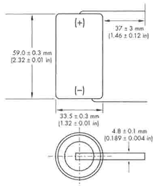
overall dimensions
