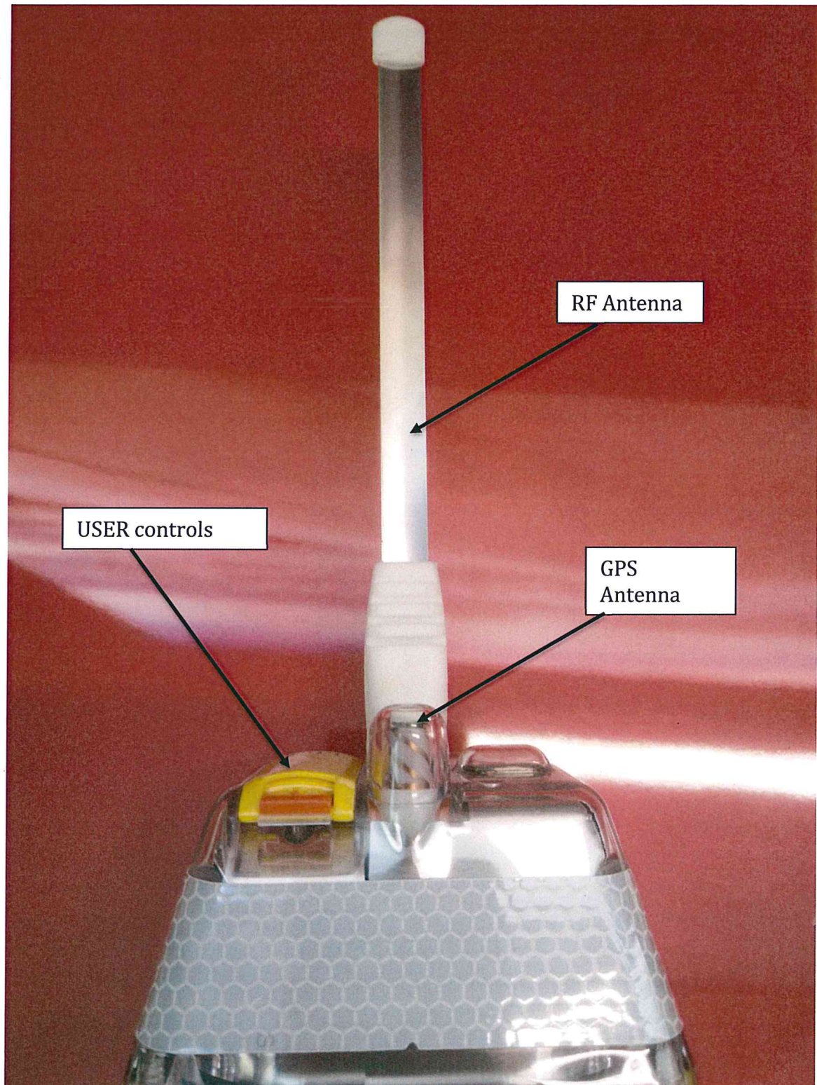
Figure 10 User controls and antennas – front view
