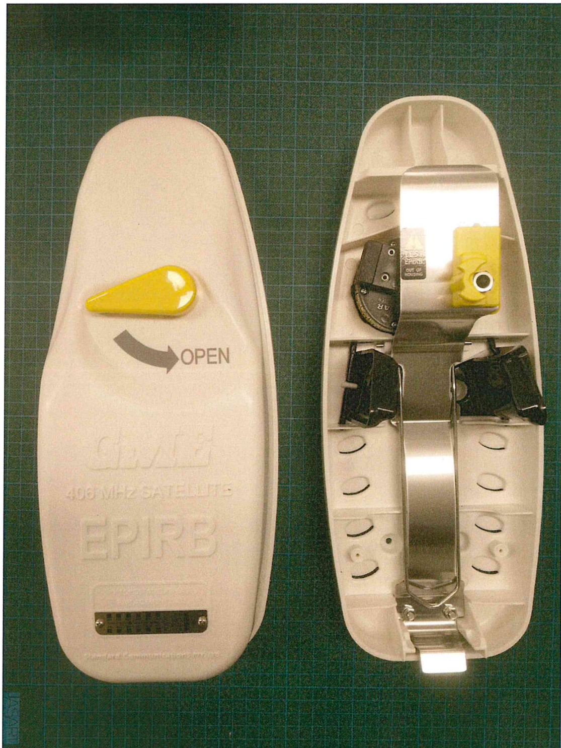
Figure 7 EPIRB Float-Free (FF) Housing - open
