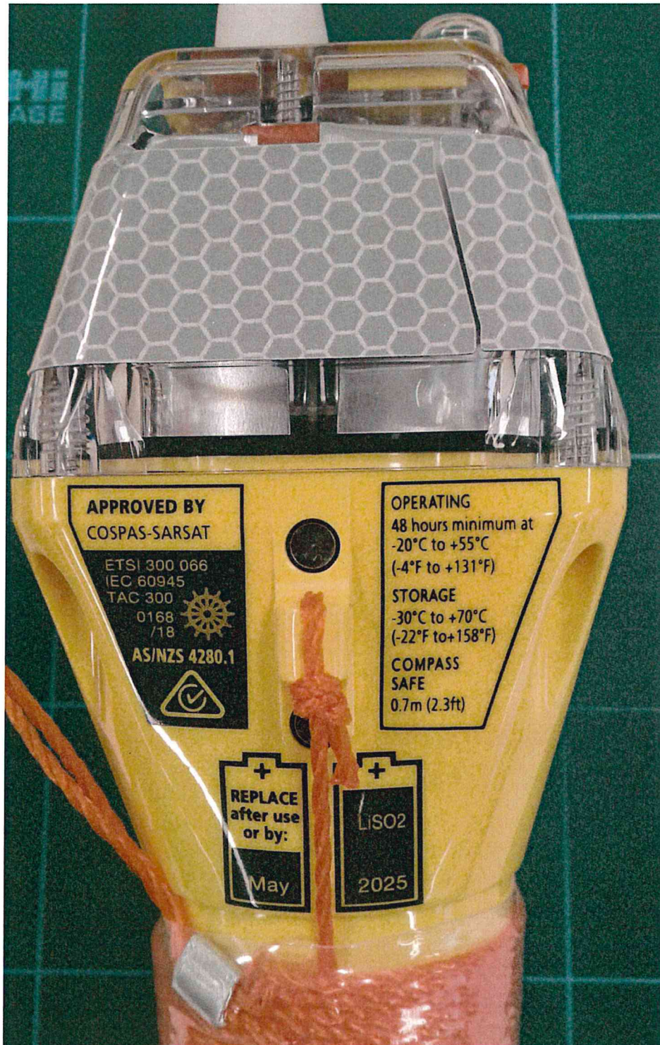
Figure 6 EPIRB face E – after laser etching
