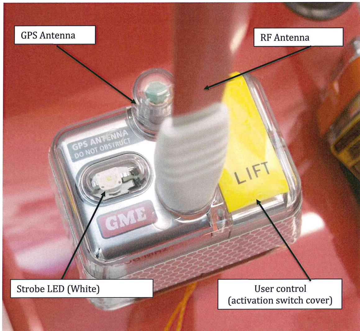
Figure 11 User controls and antennas – alternative view
