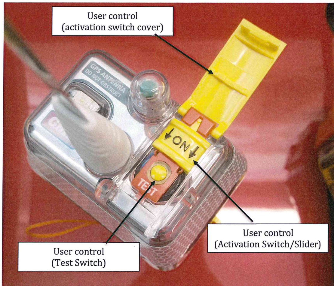
Figure 12 User controls – “Test Switch” and “Activation Switch”
