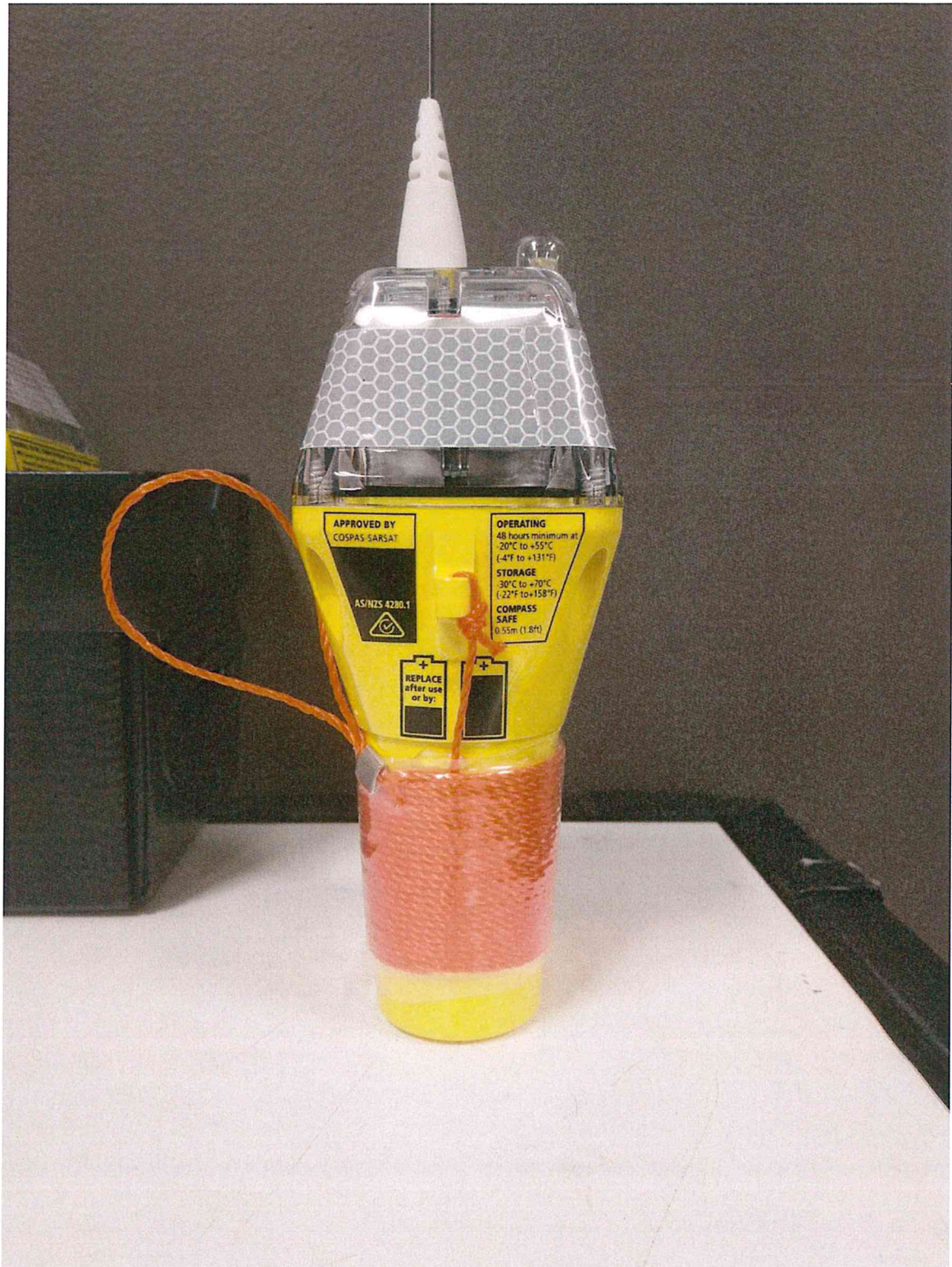
Figure 5 EPIRB face E – before laser etching
