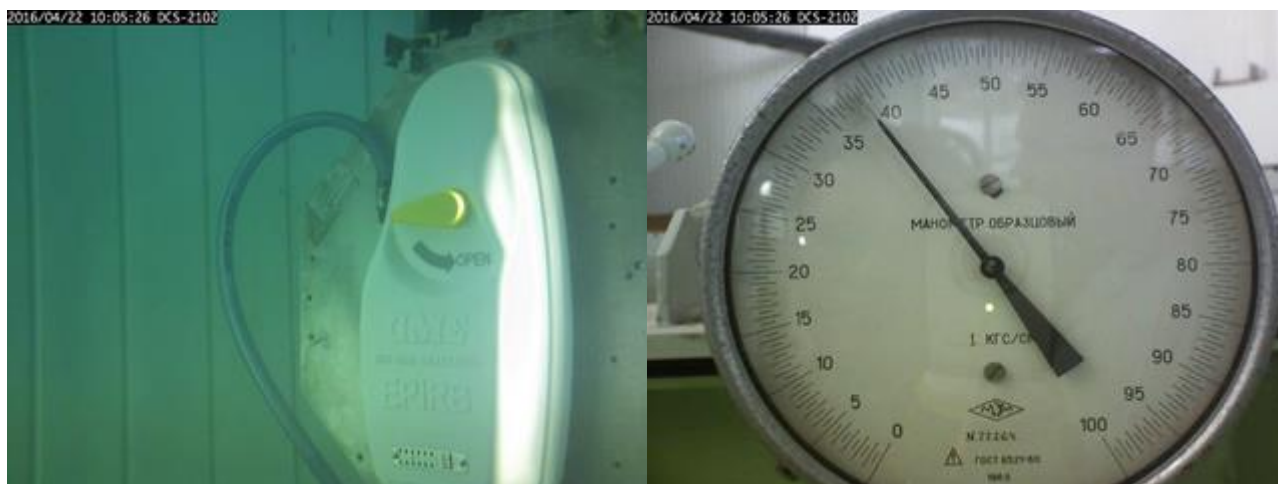
Figure 30.1 – The satellite EPIRB automatically released at normal orientation after maintained at minimum storage temperature
