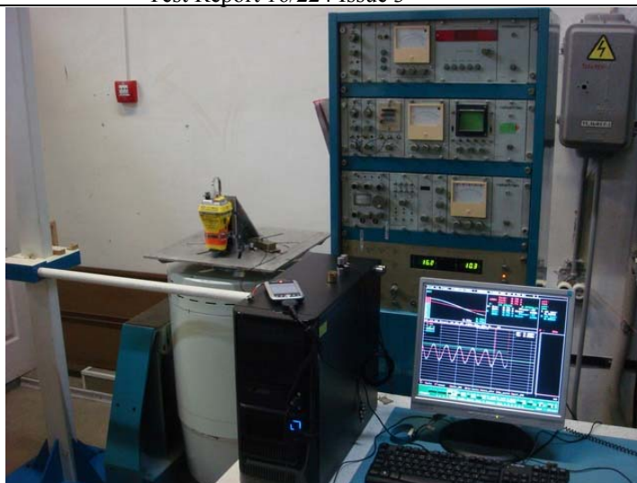
Figure 4.1 - General view of the test site vertical Z vibration (MT603G)
