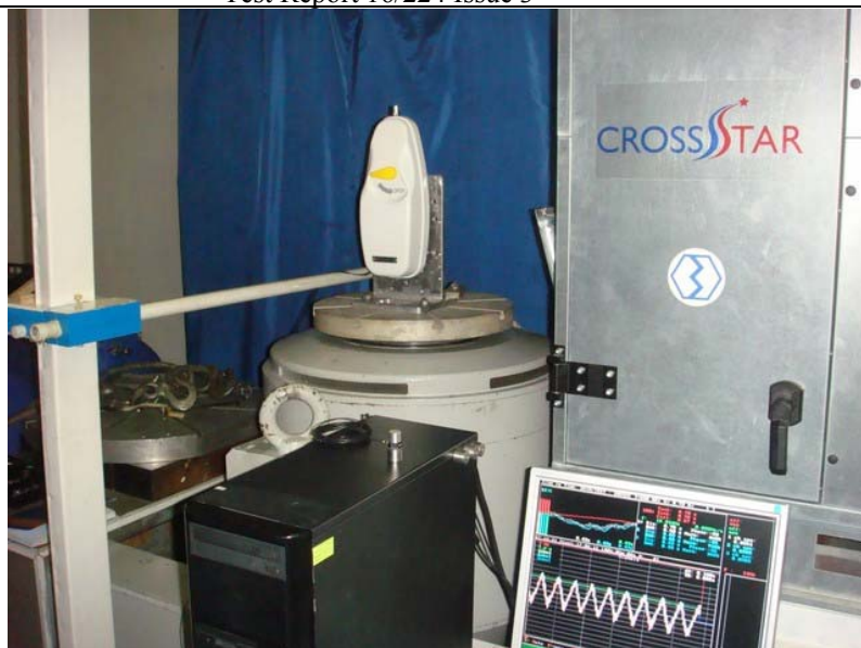
Figure 4.4 - General view of the test site vertical Z vibration (MT603FG)
