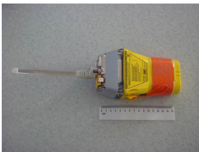
Figure 5.4 – View of the MT603G upon completion of the bump test
