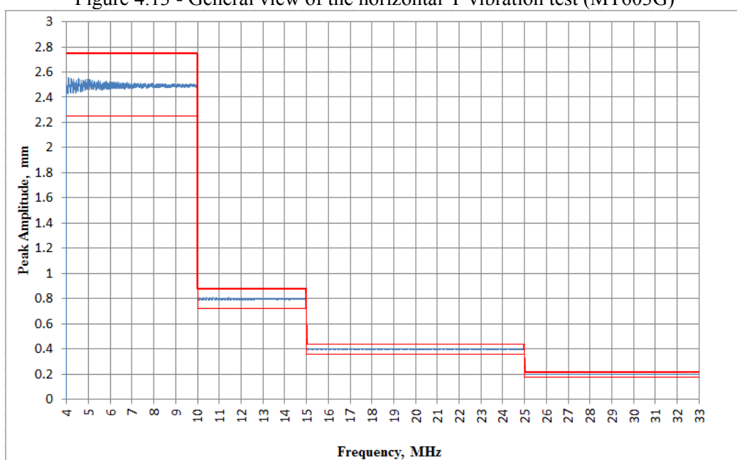
Figure 4.14 - Peak Amplitude vs. frequency during first sweep on horizontal axis Y (MT603G)
