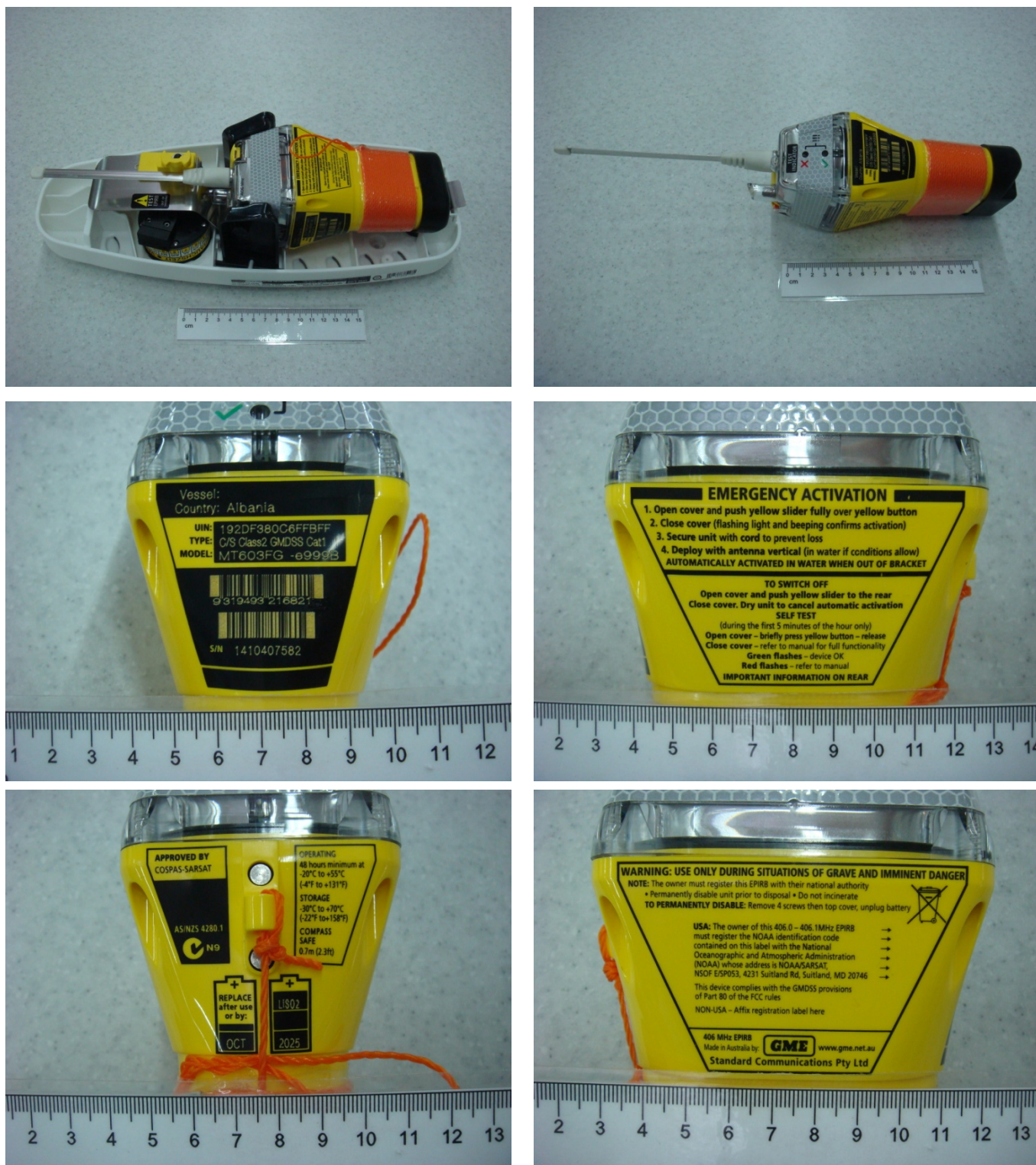
Figure 1.2 – View of MT603FG
