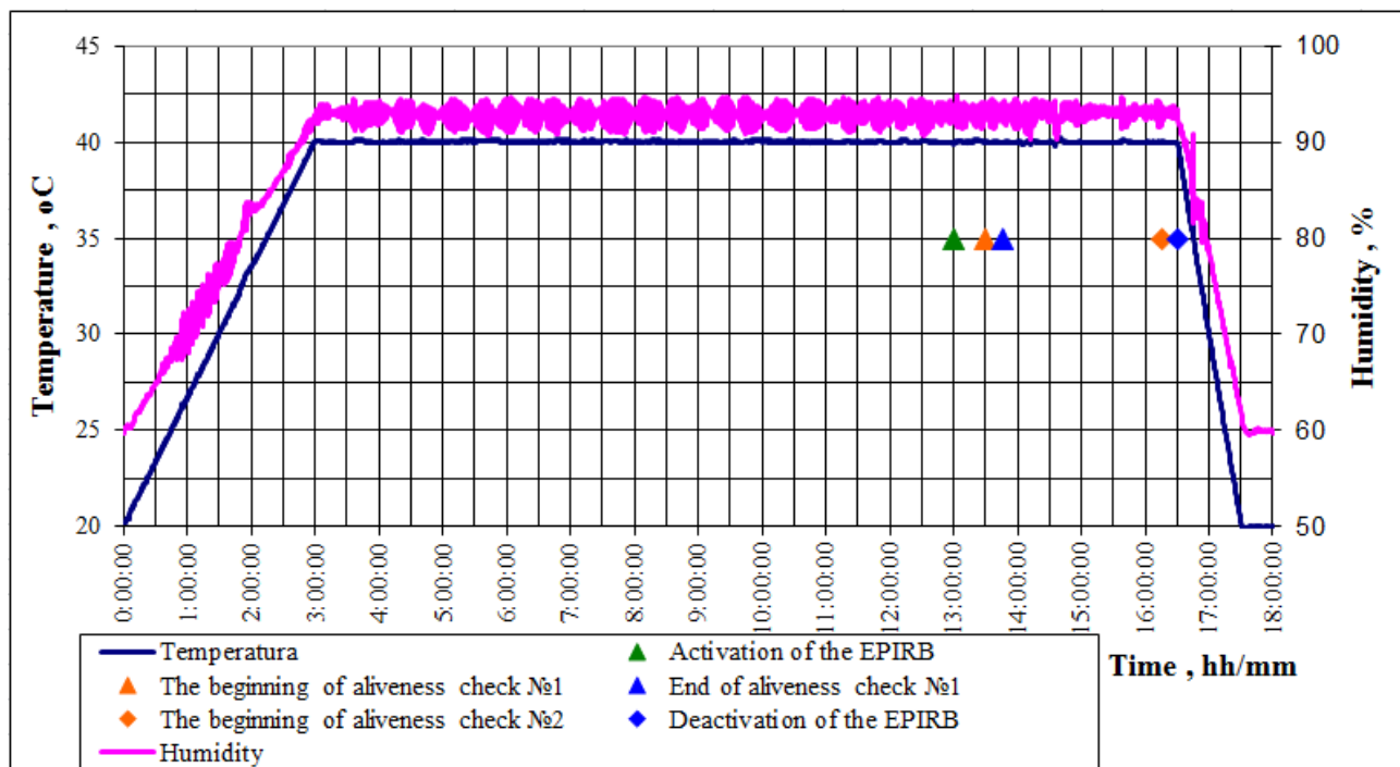
Figure 3.2 – Damp heat cycle conditions plot
