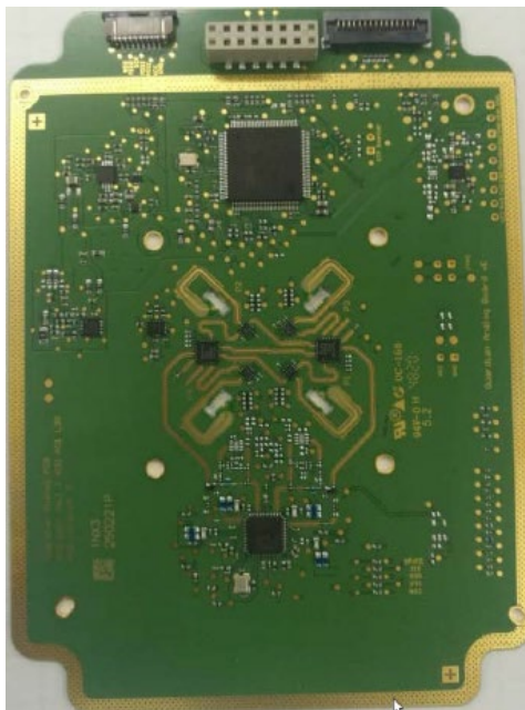
Analog PCBA, Top and Bottom (same Analog PCBA is used for both tools)
