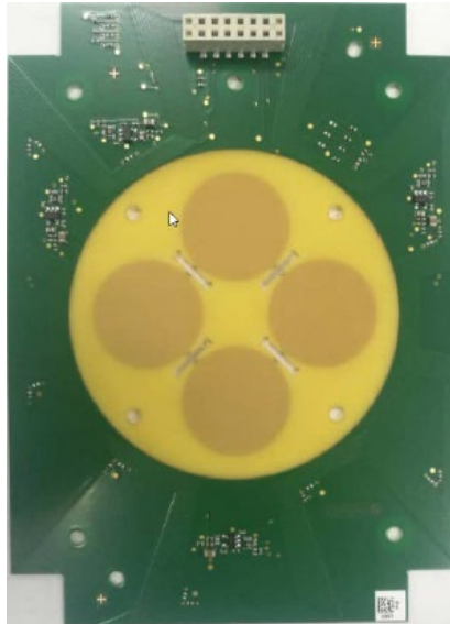
Sensor PCBA, Top and Bottom (same Sensor PCBA is used for both tools)
