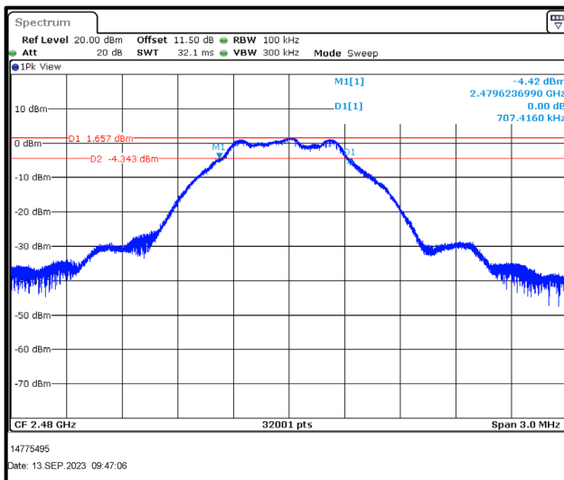
Top Channel
