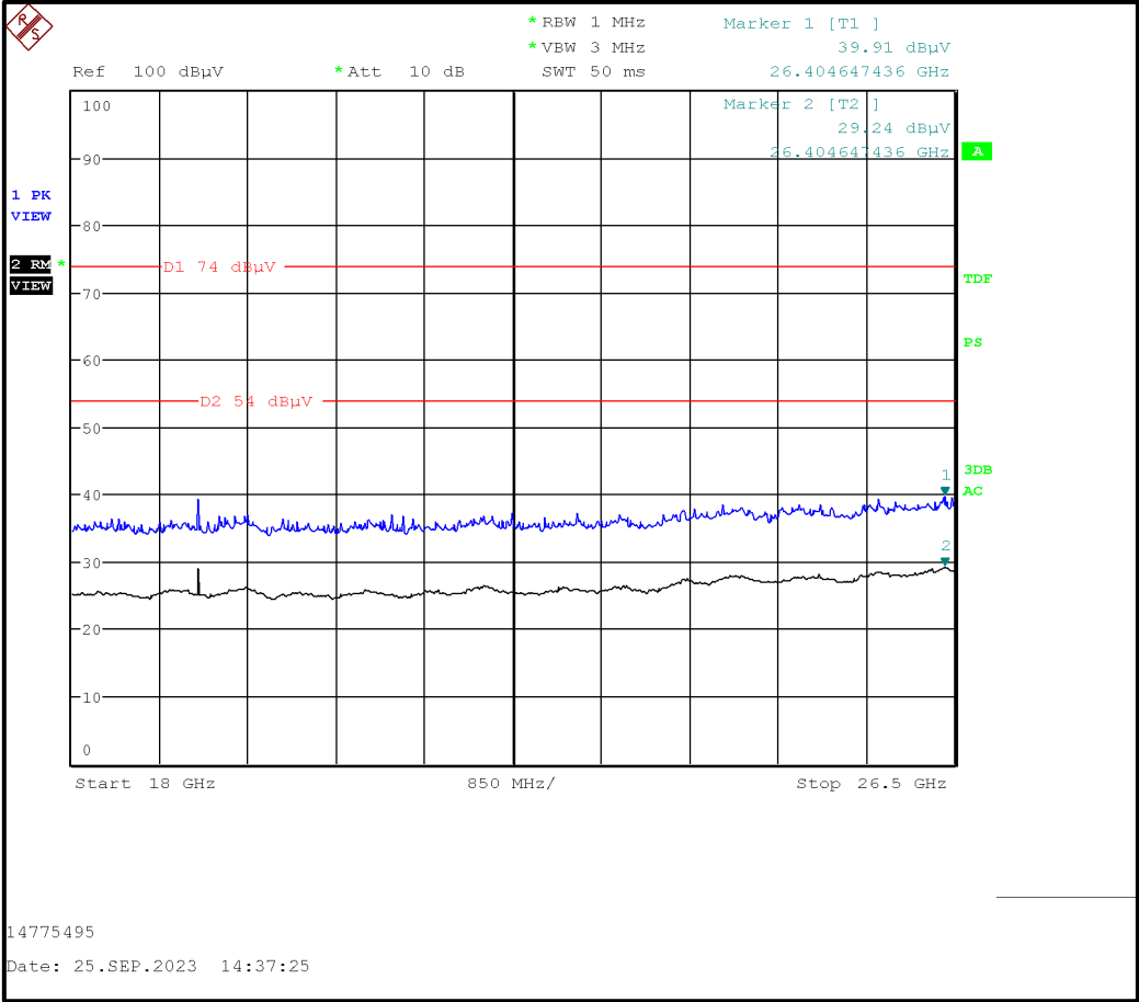
Plot: 18 GHz – 26.5 GHz: BT-LE / 1 Mbps / PRBS9 / PWR 5 / Bottom Channel
