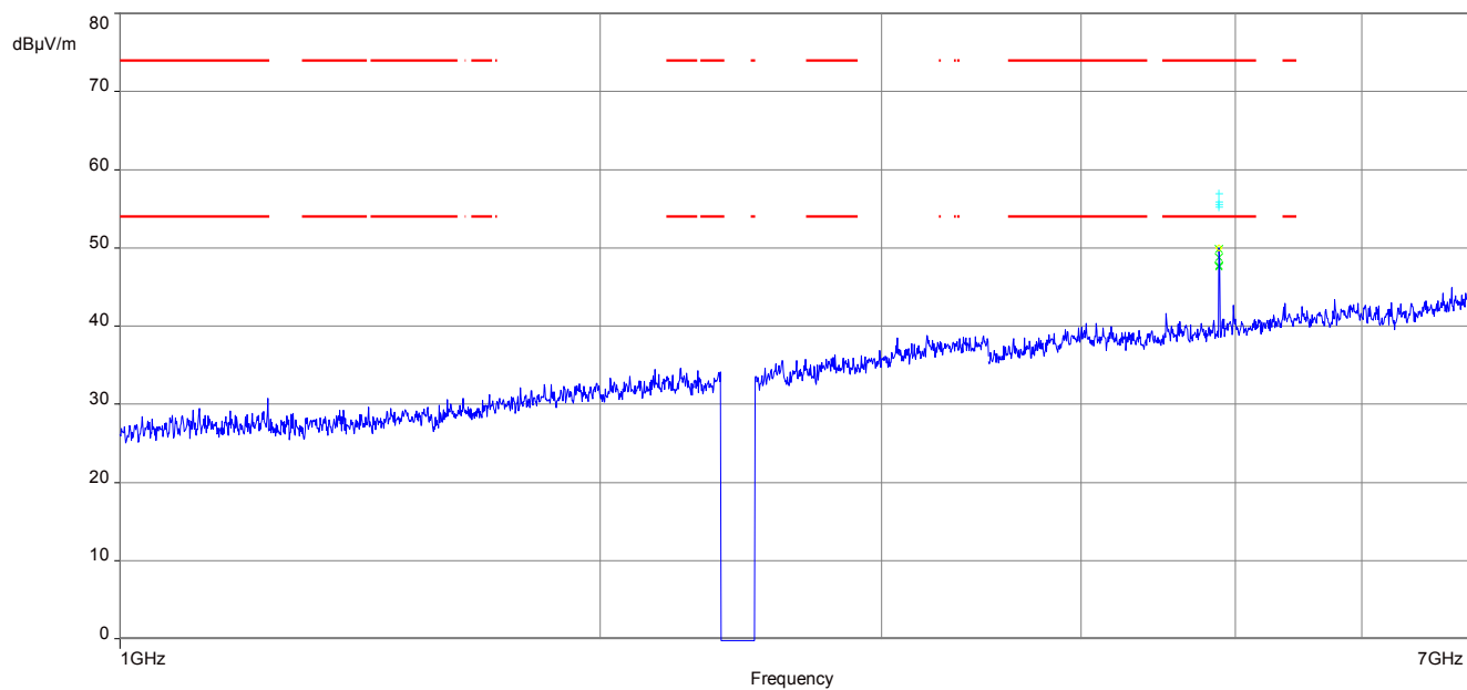
Plot 5: 1 GHz to 7 GHz, TX mode, channel 19, vertical & horizontal polarization
