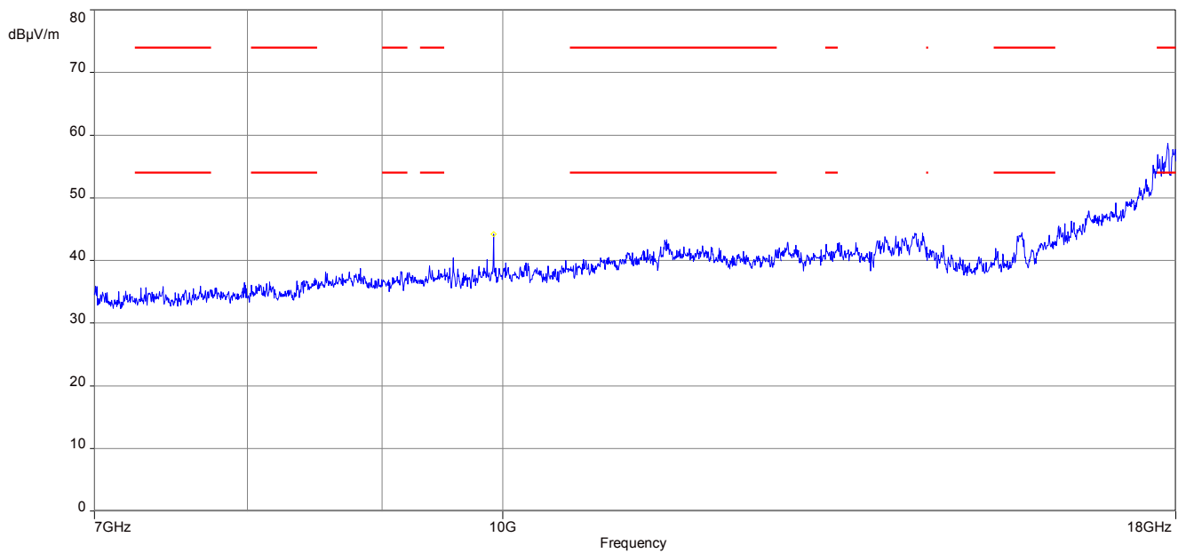
Plot 10: 7 GHz to 18 GHz, TX mode, channel 39, vertical & horizontal polarization
