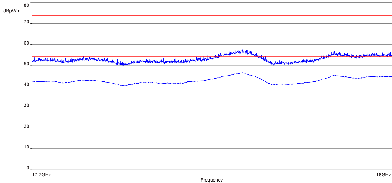
Plot 7: 17.7 GHz to 18 GHz, TX mode, channel 19, vertical & horizontal polarization
