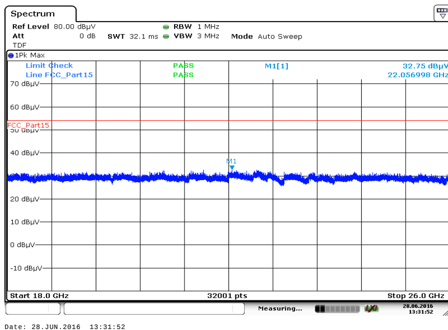
Plot 12: 18 GHz to 26 GHz, TX mode, channel 39, vertical & horizontal polarization
