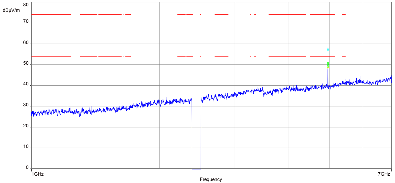
Plot 9: 1 GHz to 7 GHz, TX mode, channel 39, vertical & horizontal polarization
