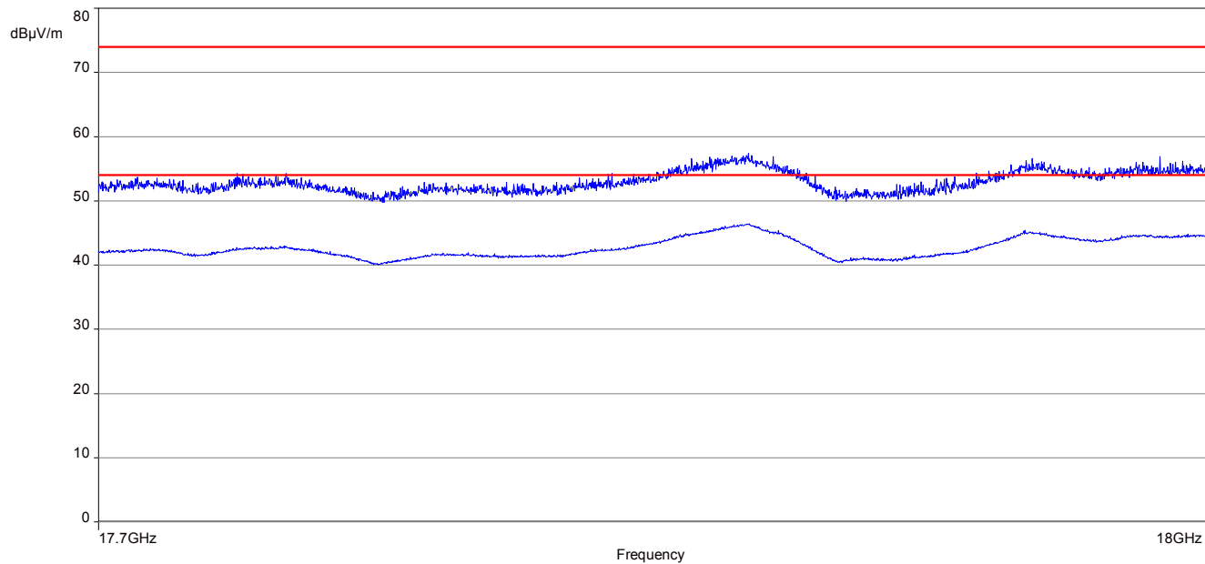
Plot 11: 17.7 GHz to 18 GHz, TX mode, channel 39, vertical & horizontal polarization
