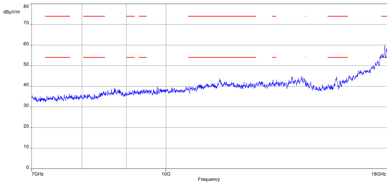
Plot 6: 7 GHz to 18 GHz, TX mode, channel 19, vertical & horizontal polarization
