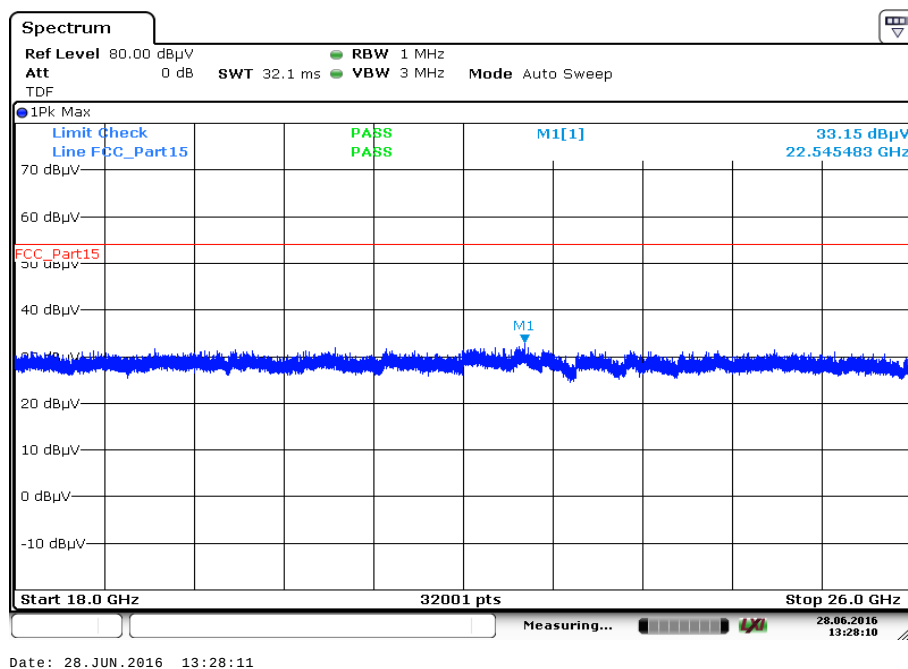
Plot 8: 18 GHz to 26 GHz, TX mode, channel 19, vertical & horizontal polarization
