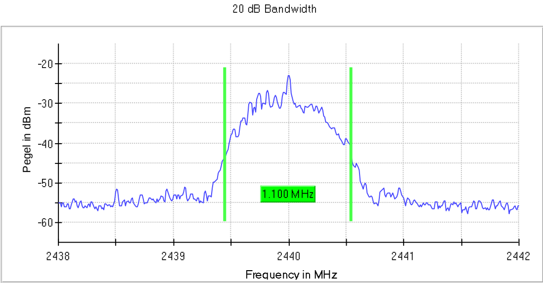
20dB-BW, 2440 MHz
