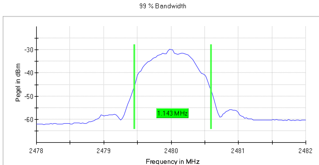
99%-BW, 2480 MHz
