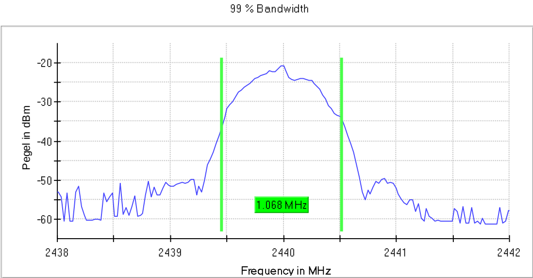
99%-BW, 2440 MHz
