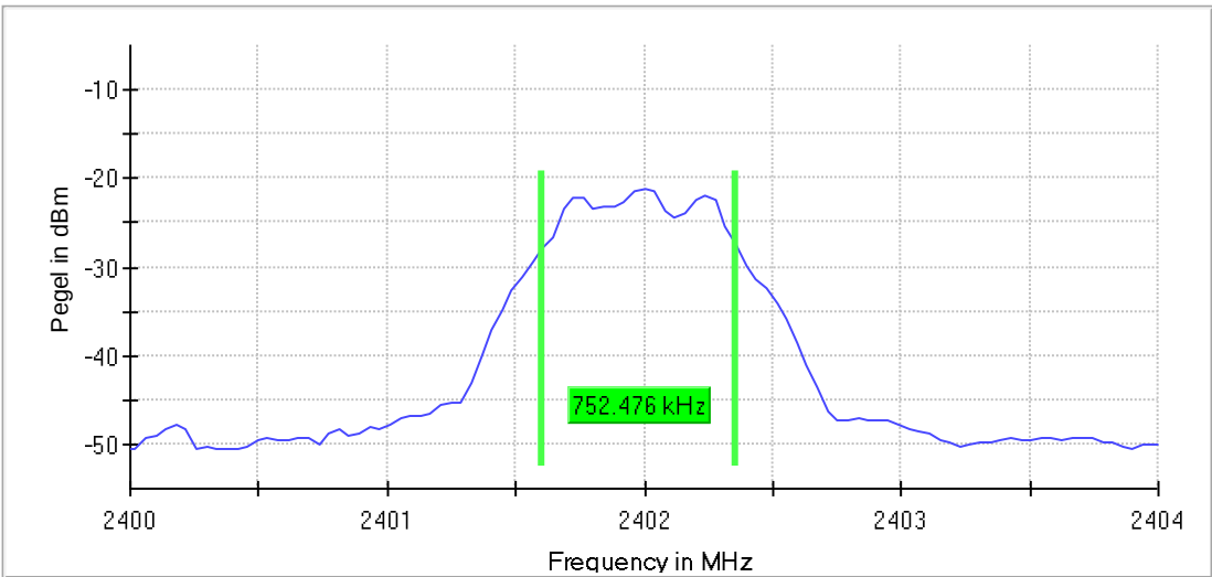
6dB-BW, 2402 MHz
