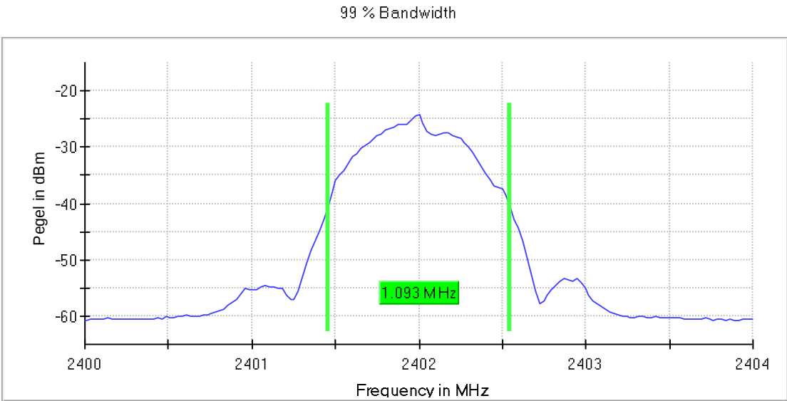
99%-BW, 2402 MHz
