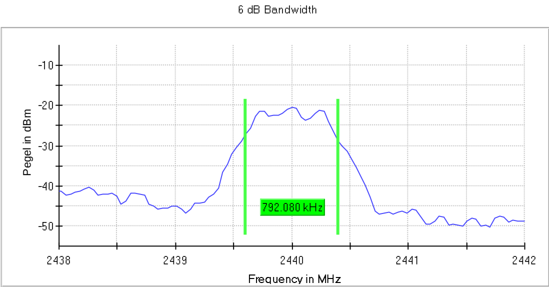
6dB-BW, 2440 MHz
