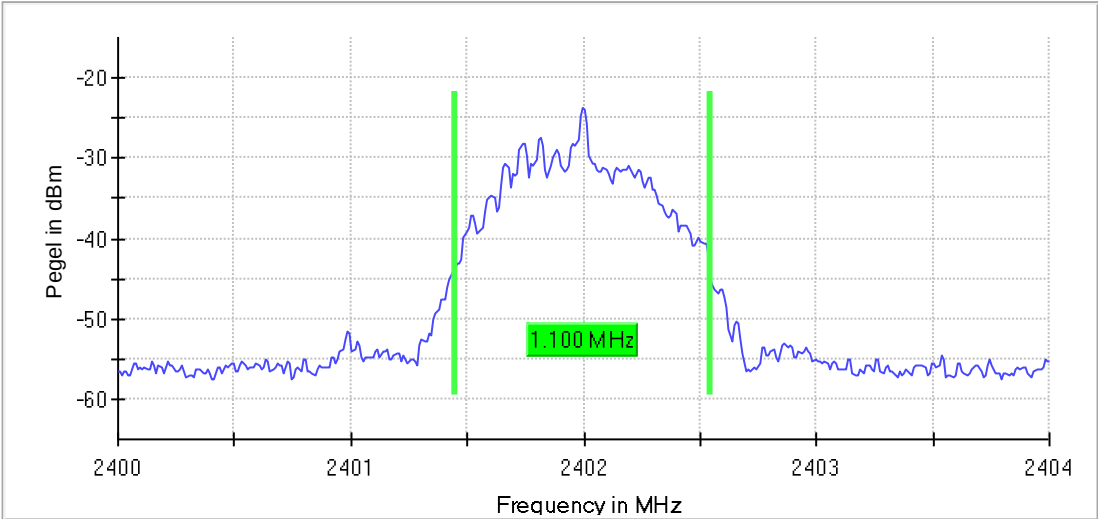
20dB-BW, 2402 MHz,
