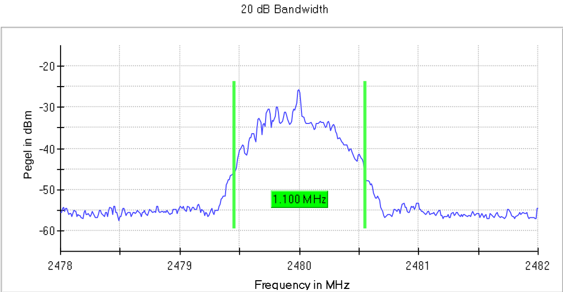
20dB-BW, 2480 MHz
