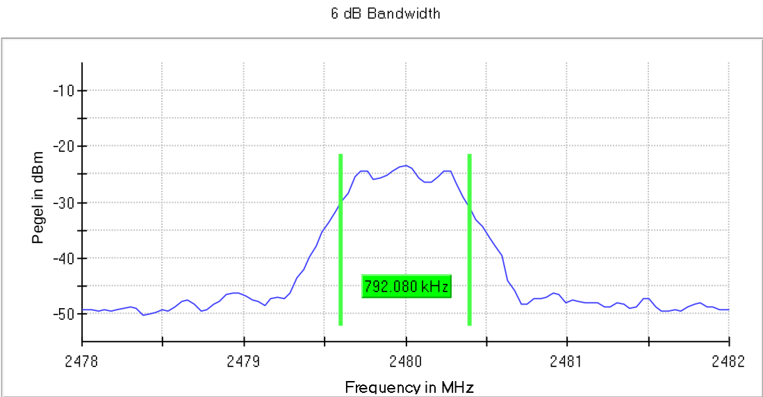
6dB-BW, 2480 MHz
