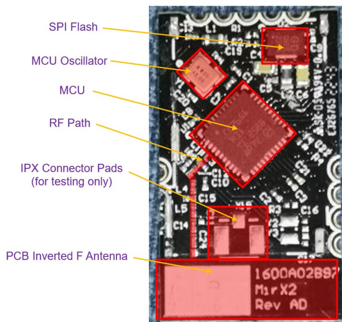
Key components layout (Top View)
