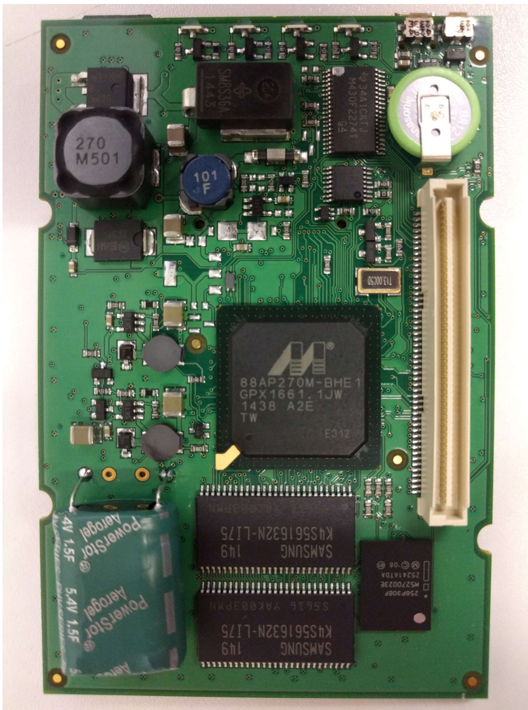
CPU PCB Bottom Side
