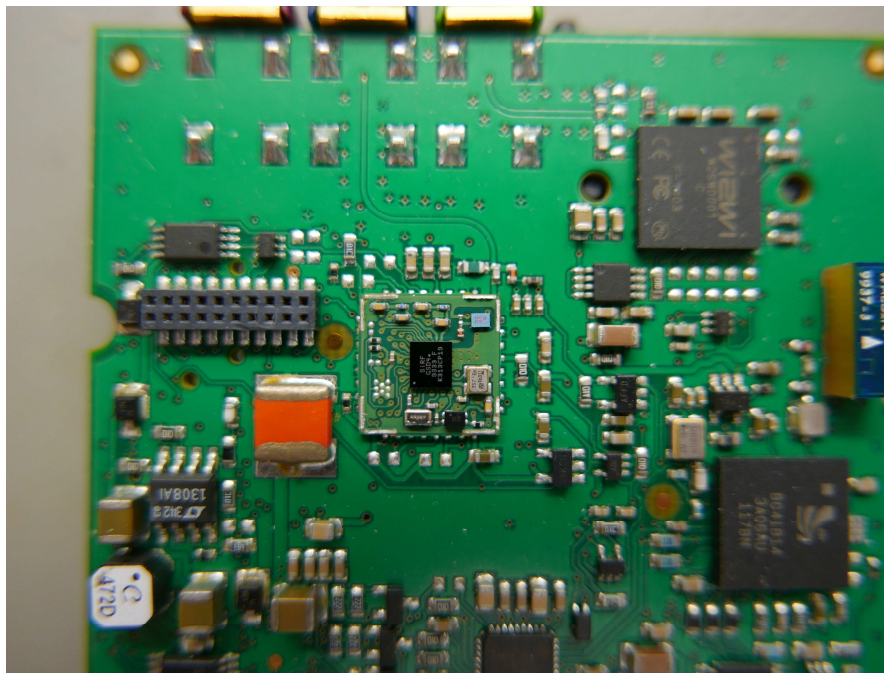
Telit JF2 GPS Module (Shield Removed)
