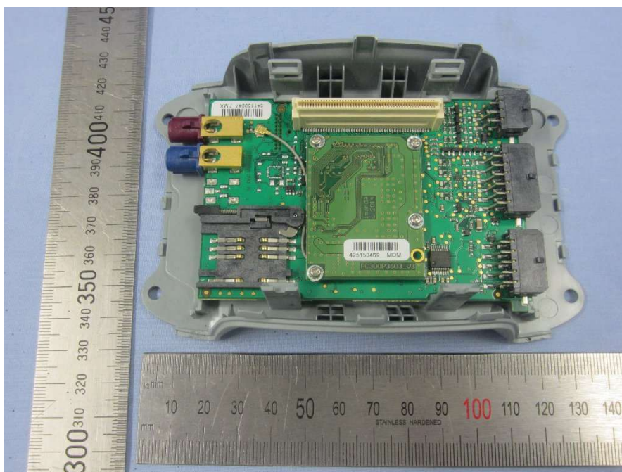
CPU (Top) PCB Removed Showing FMX PCB
