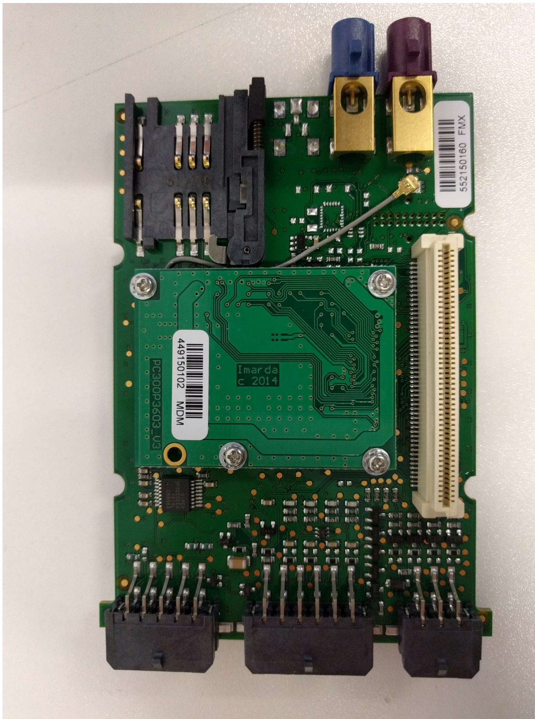
FMX Top Side
