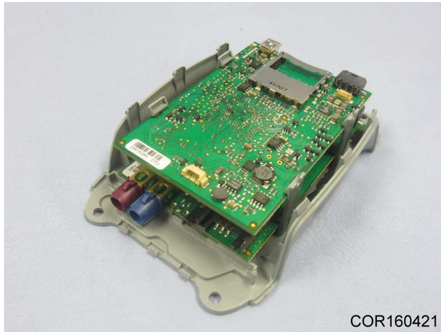
Cover Removed (Showing CPU & FMX PCBs)
