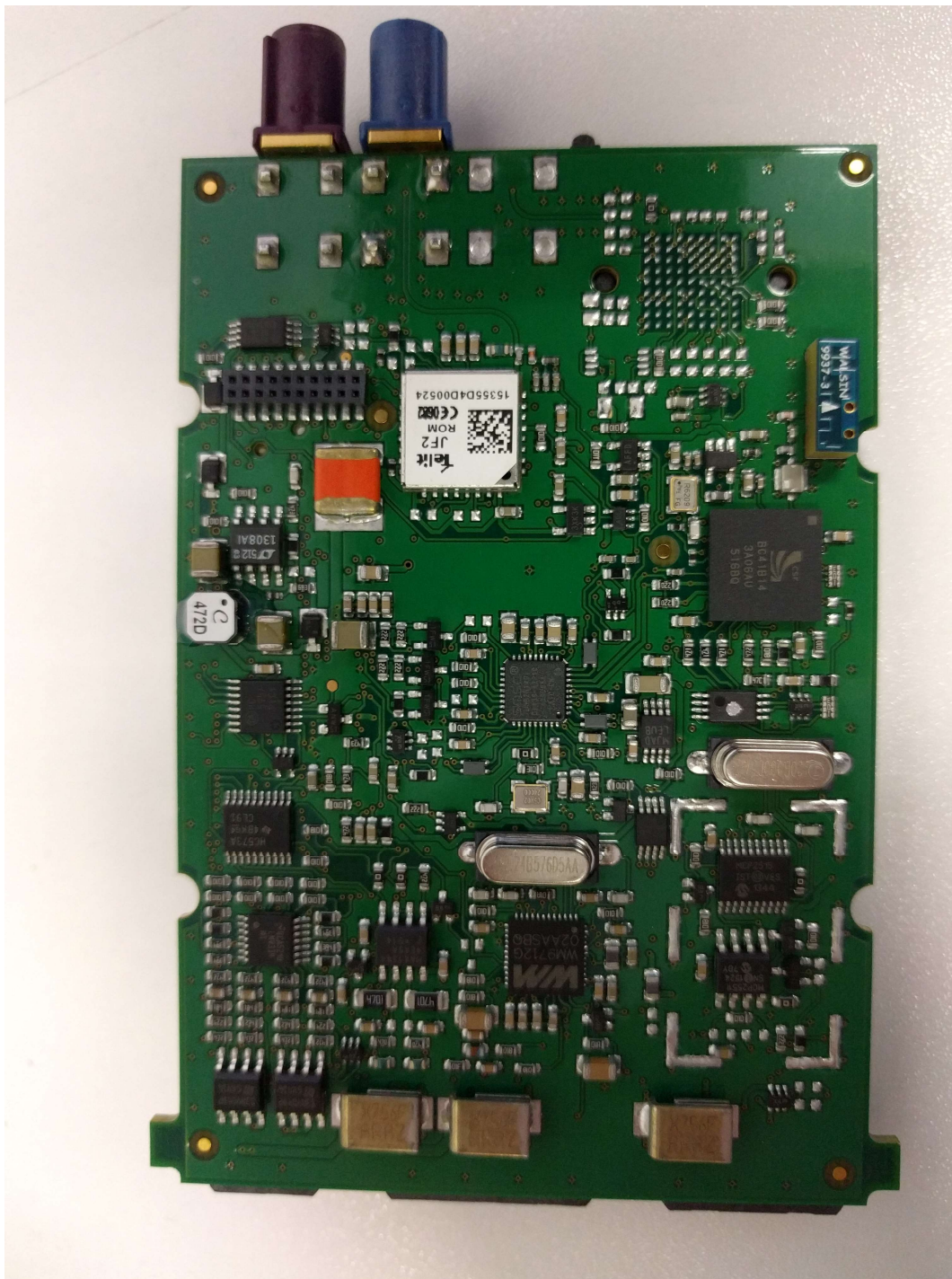
FMX Bottom Side
