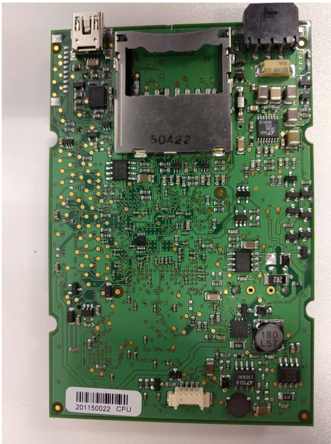
CPU PCB Top Side
