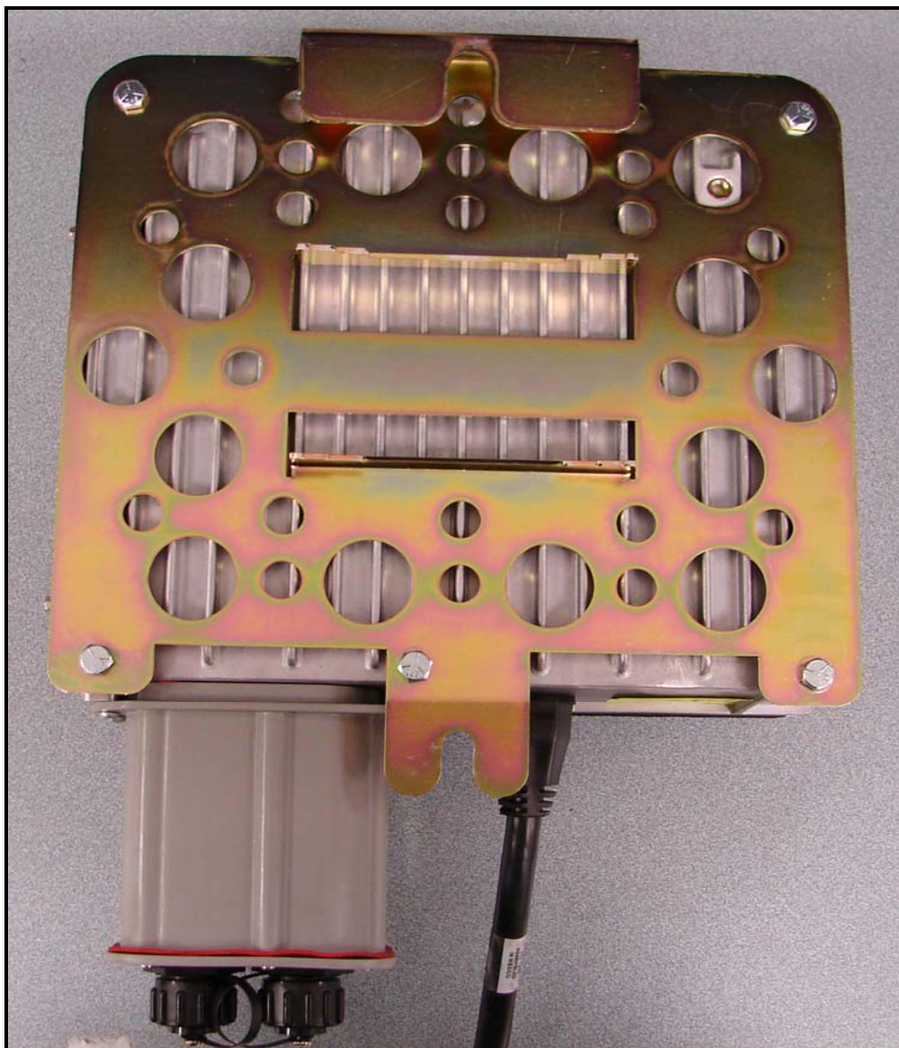
Photograph EP-2: External Photo of CT Backhaul-Point – View of Bottom Side
