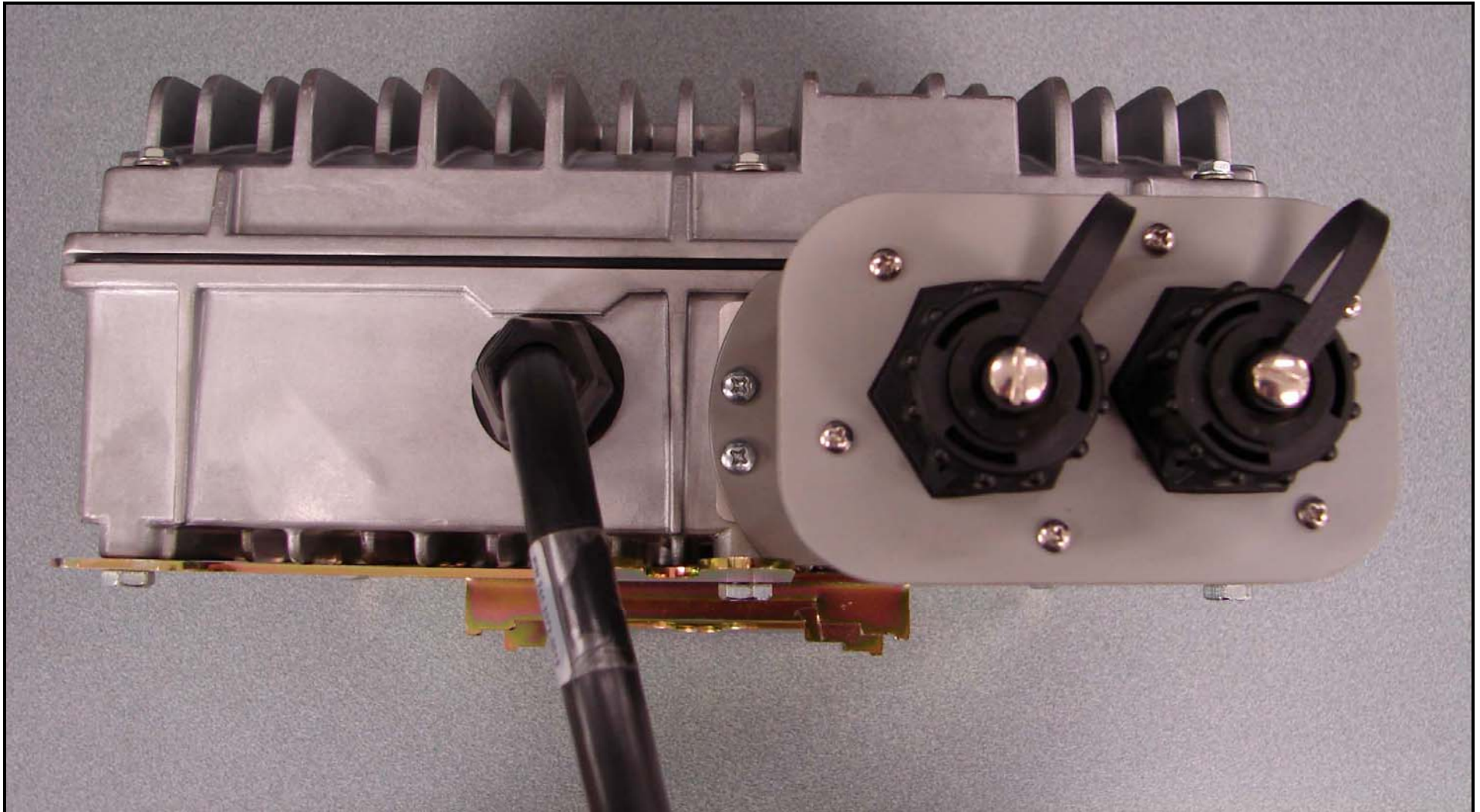
Photograph EP-3: External Photo of CT Backhaul-Point – Connectors
