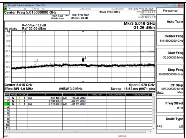
Band5 1.4MHz QPSK RB1 0 CH20525 below 18G
