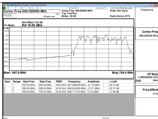
Band12 1.4MHz QPSK RB6 0 CH23017
