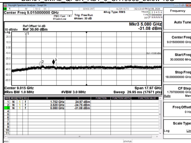
Band4 3MHz QPSK RB1 0 CH20385 below 18G
