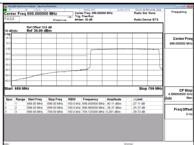
Band12 10MHz QPSK RB50 0 CH23060
