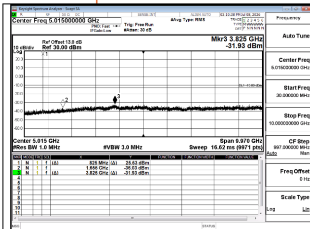
Band5 1.4MHz QPSK RB1 0 CH20407 below 18G
