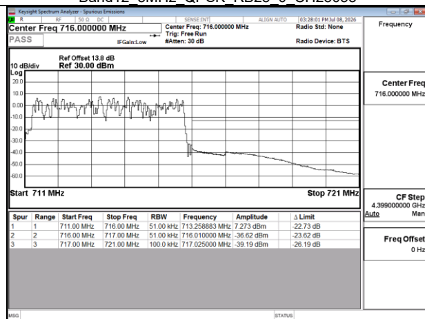
Band12 5MHz QPSK RB25 0 CH23155
