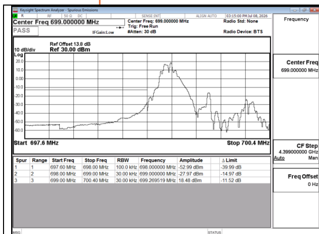
Band12 1.4MHz QPSK RB1 0 CH23017
