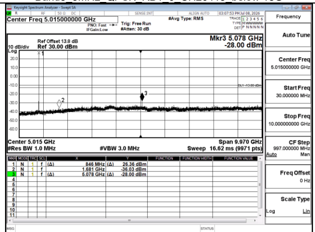
Band5 3MHz QPSK RB1 0 CH20635 below 18G
