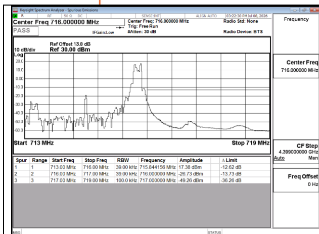
Band12 3MHz QPSK RB1 14 CH23165
