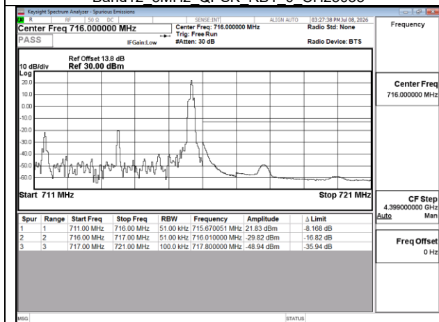
Band12 5MHz QPSK RB1 24 CH23155
