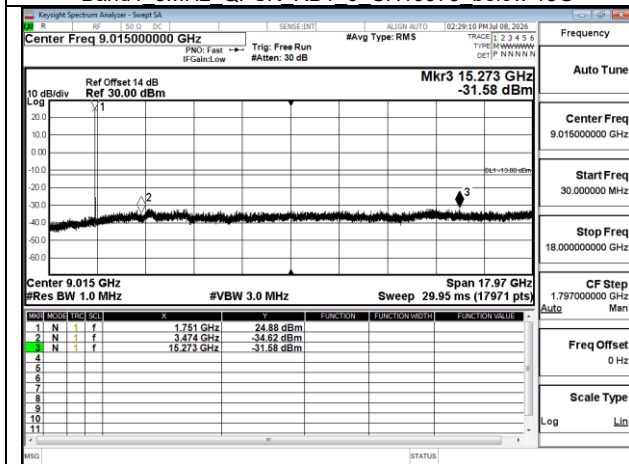
Band4 5MHz QPSK RB1 0 CH20375 below 18G
