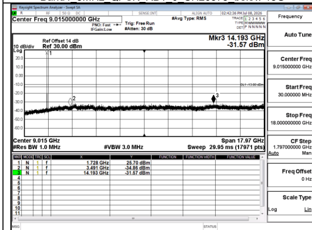
Band4 10MHz QPSK RB1 0 CH20175 below 18G
