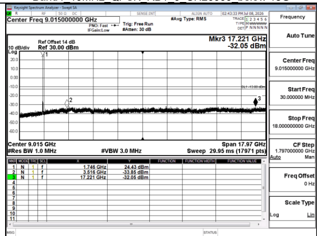
Band4 10MHz QPSK RB1 0 CH20350 below 18G
