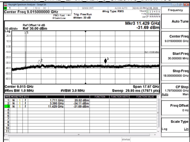
Band4 10MHz QPSK RB1 0 CH20000 below 18G
