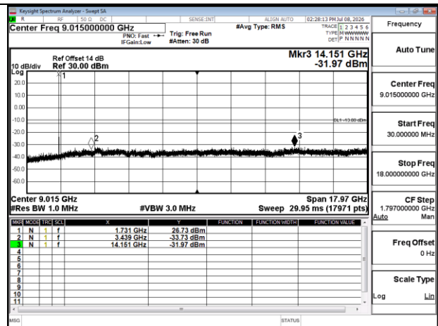
Band4 5MHz QPSK RB1 0 CH20175 below 18G
