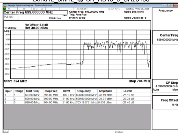
Band12 5MHz QPSK RB25 0 CH23035
