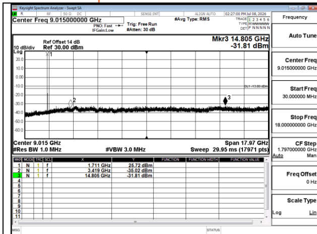
Band4 5MHz QPSK RB1 0 CH19975 below 18G
