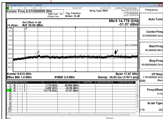
Band4 1.4MHz QPSK RB1 0 CH19957 below 18G
