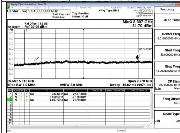
Band13 5MHz QPSK RB1 0 CH23255 below 18G
