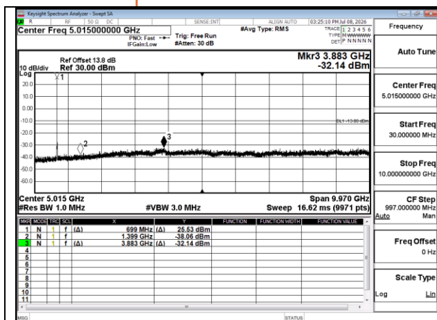
Band12 5MHz QPSK RB1 0 CH23035 below 18G
