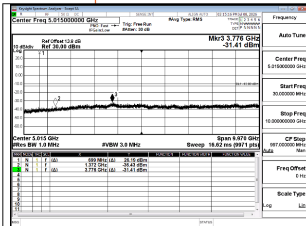
Band12 1.4MHz QPSK RB1 0 CH23017 below 18G
