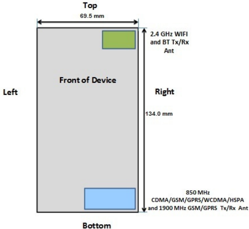
Figure 1-2 DUT Antenna Locations
