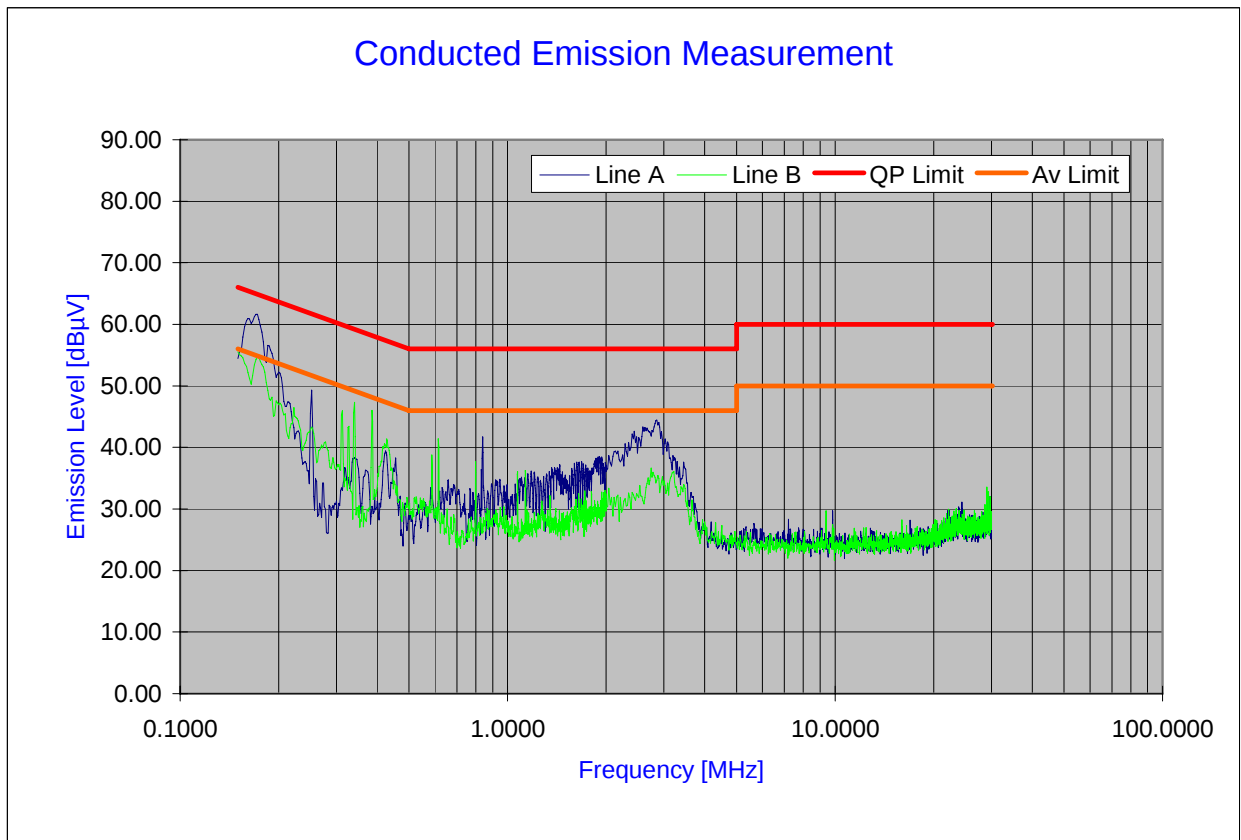
Plot 6-24. Line Conducted Plot with Bluetooth
