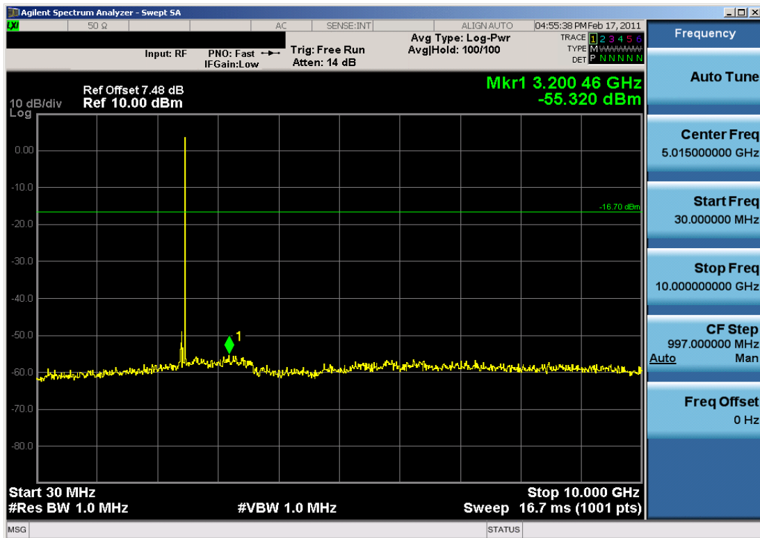
Plot 6-18. Conducted Spurious Plot (Bluetooth, 2Mbps – Ch. 0)
