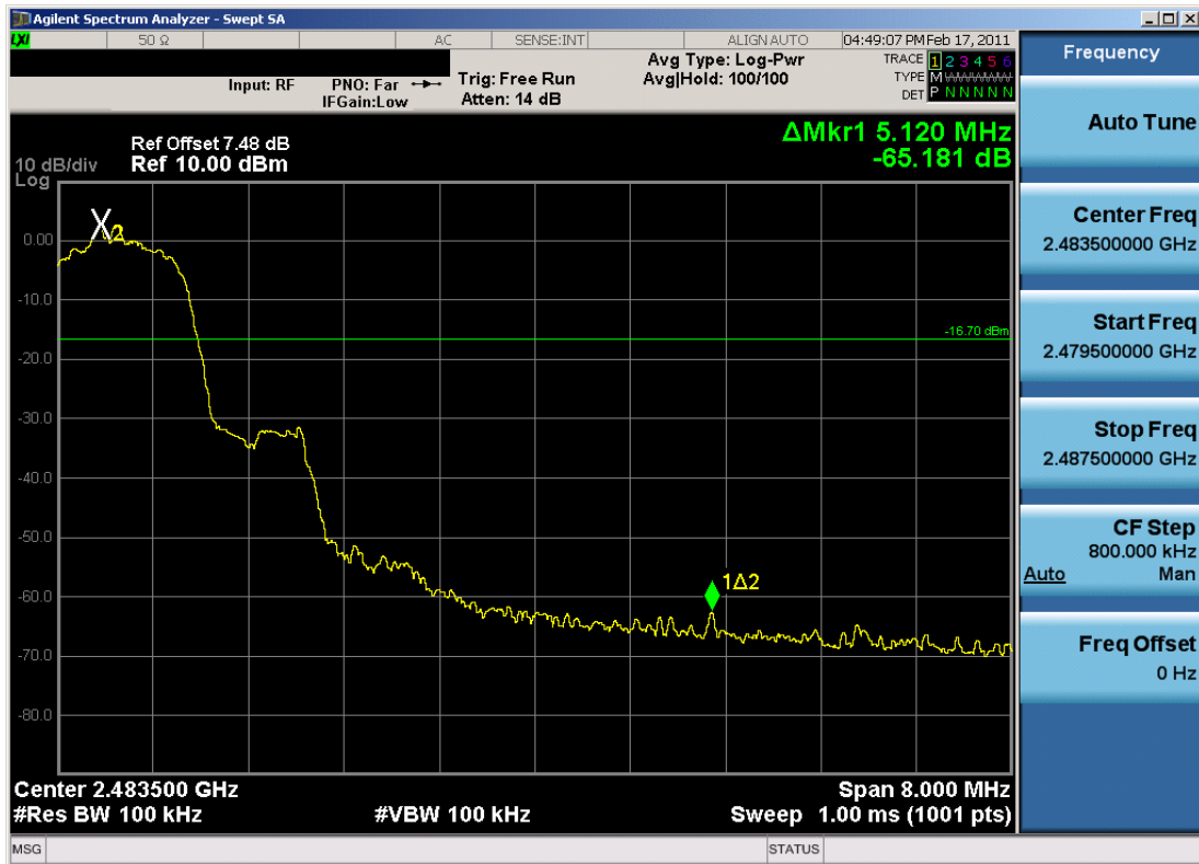
Plot 6-13. Band Edge Plot (Bluetooth, 2Mbps – Ch. 78)
