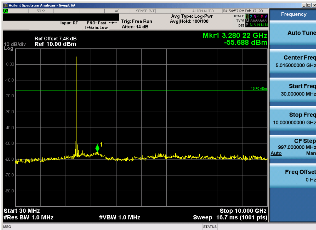
Plot 6-20. Conducted Spurious Plot (Bluetooth, 2Mbps – Ch. 39)
