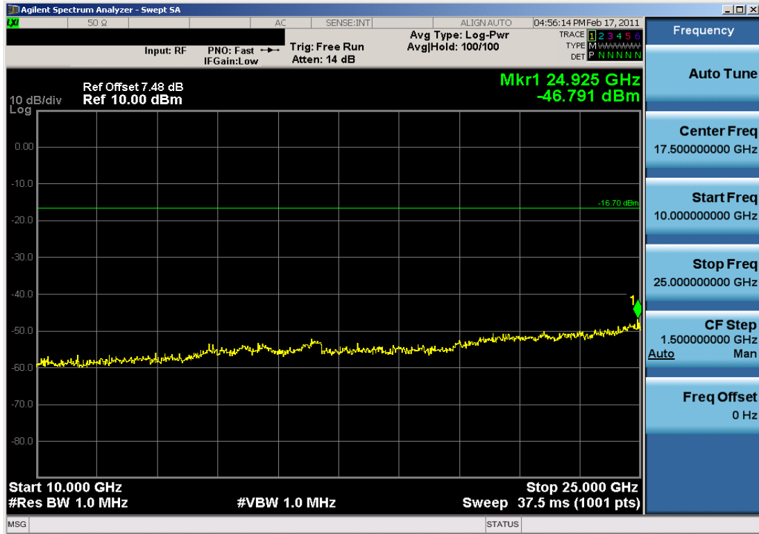
Plot 6-19. Conducted Spurious Plot (Bluetooth, 2Mbps – Ch. 0)
