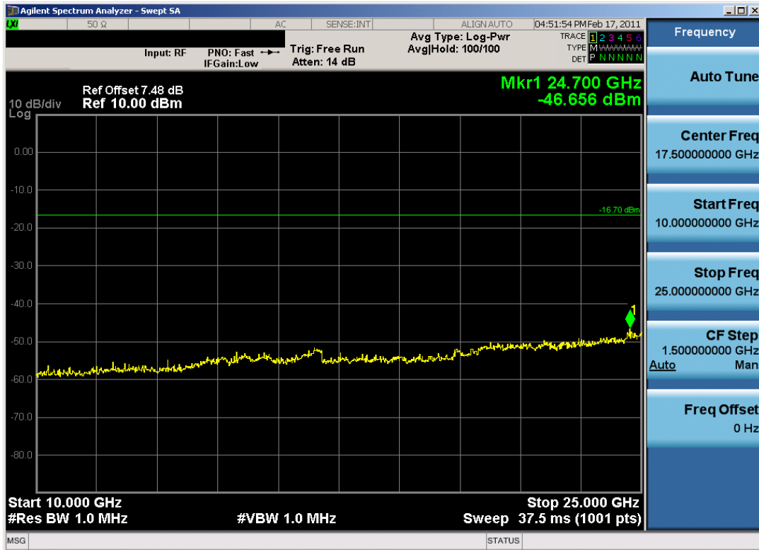
Plot 6-23. Conducted Spurious Plot (Bluetooth, 2Mbps – Ch. 78)
