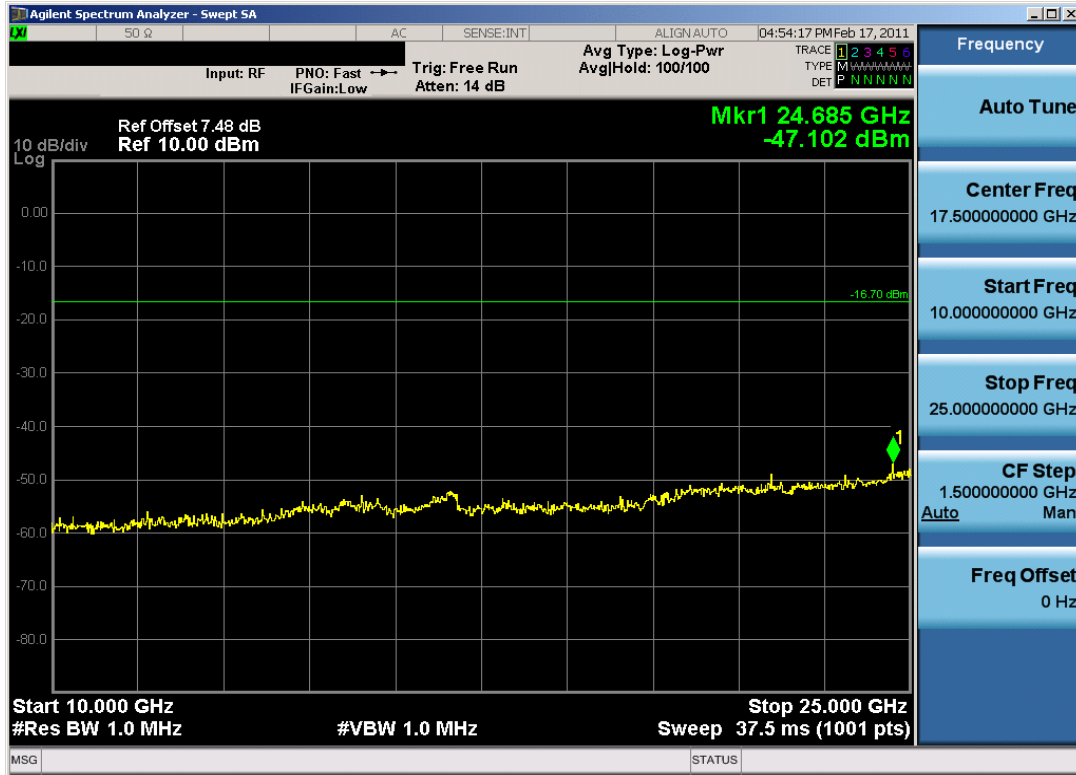
Plot 6-21. Conducted Spurious Plot (Bluetooth, 2Mbps – Ch. 39)
