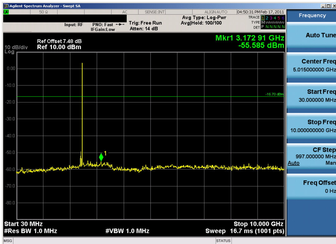
Plot 6-22. Conducted Spurious Plot (Bluetooth, 2Mbps – Ch. 78)
