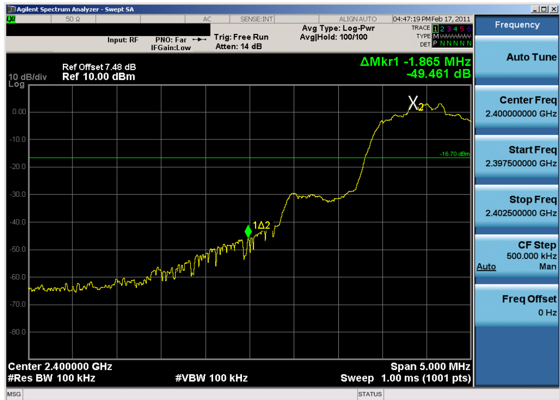
Plot 6-12. Band Edge Plot (Bluetooth, 2Mbps – Ch. 0)
