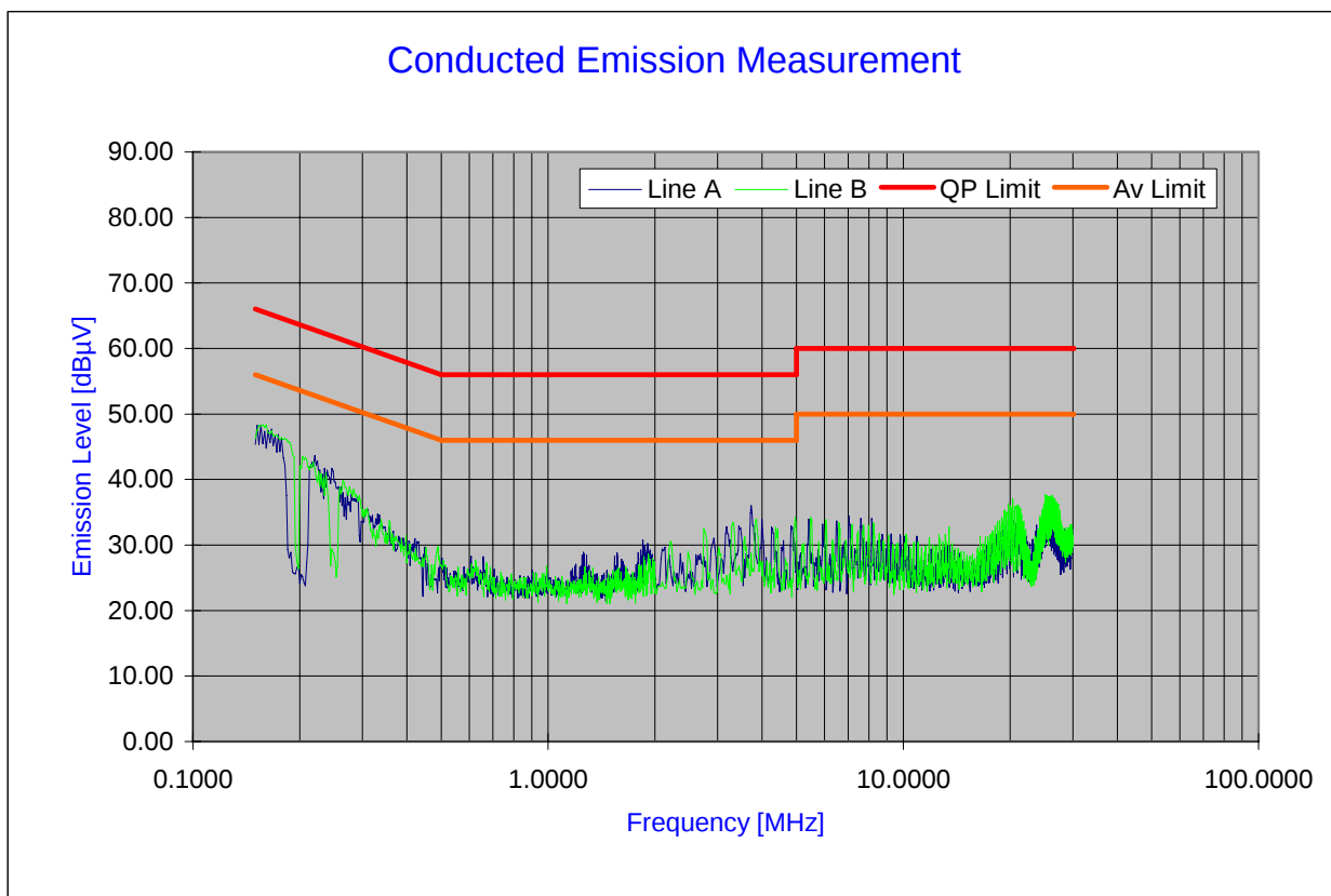
Plot 6-33. Line Conducted Plot with 802.11n
