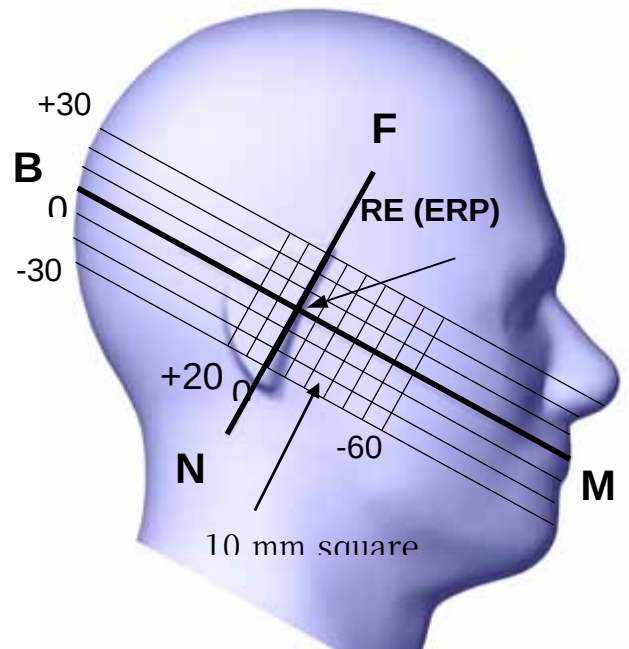
Figure 6. EUT Head Position
