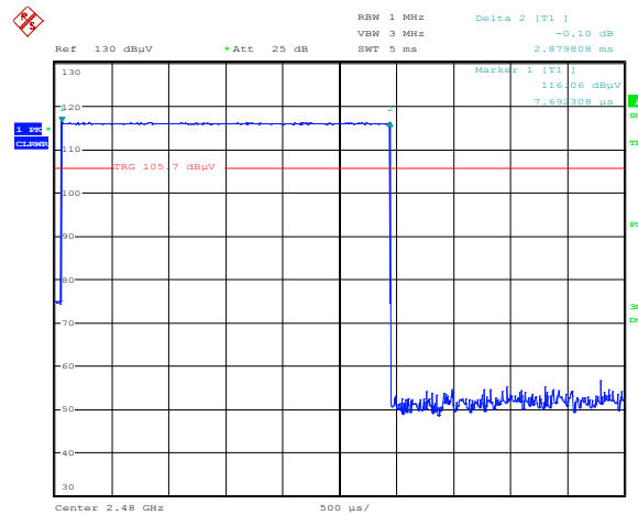
Figure 8.2-12: Pulse width at DH3
