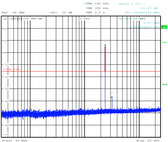
Figure 8.5-10: Conducted spurious emissions for GFSK, mid channel
