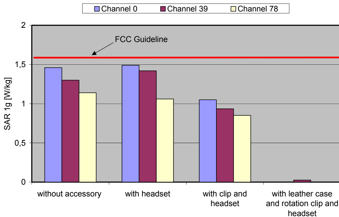
Fig. 8: The measured SAR values in body-worn configuration for the Avaya Tenovis BlueVoice L Home for the Bluetooth standard in comparison to the FCC exposure limit.
