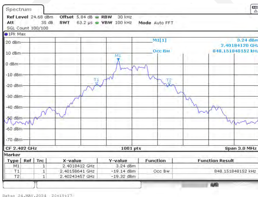
99%_Occupied_Bandwidth_NVNT_ANT1_1-DH1_2402
