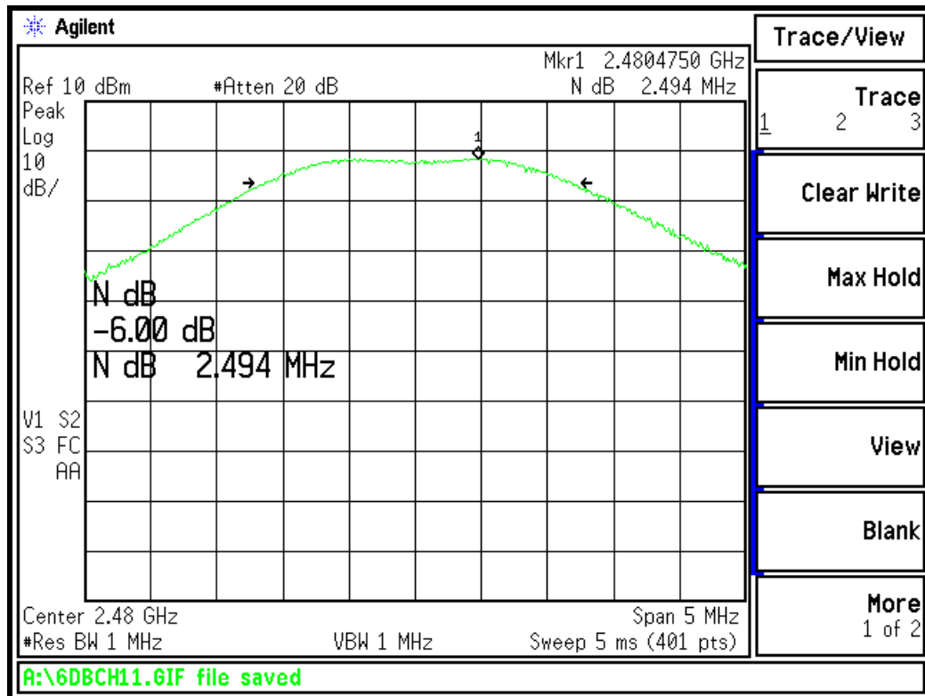
6 dB Bandwidth
