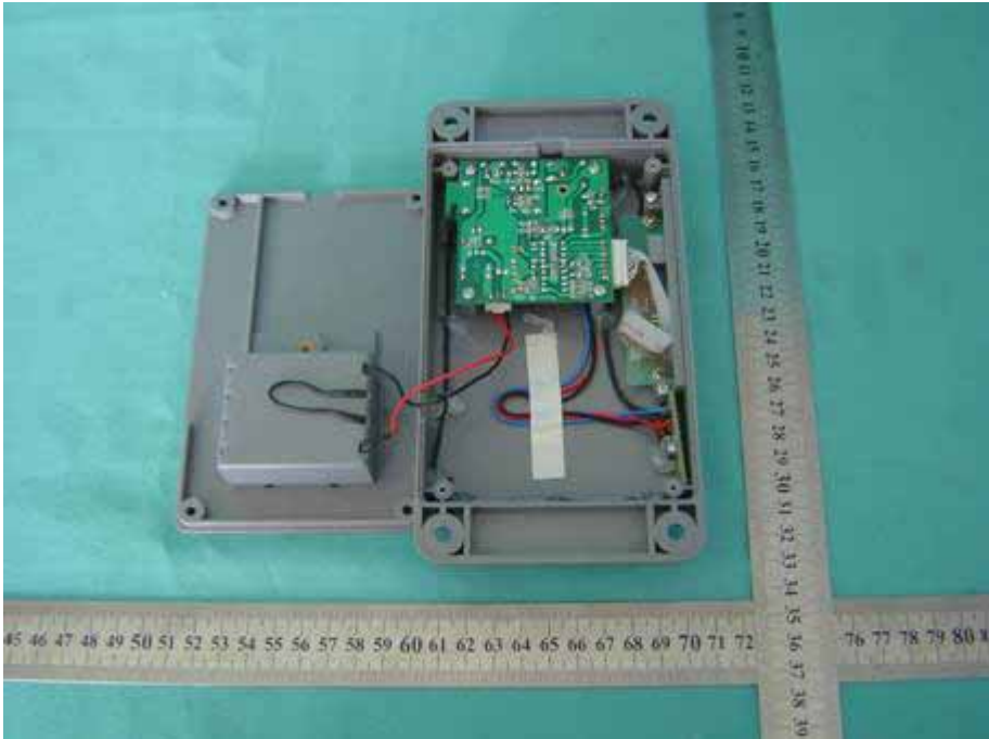
Figure 3 Main Board, Component Side
