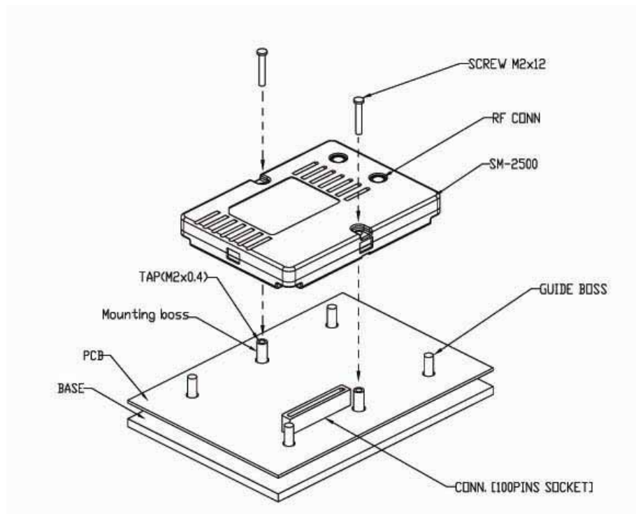
Mechanical interface
