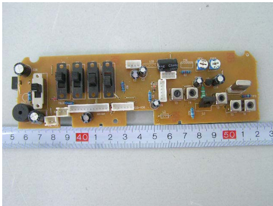
EUT – Main PCB Front View (1)
