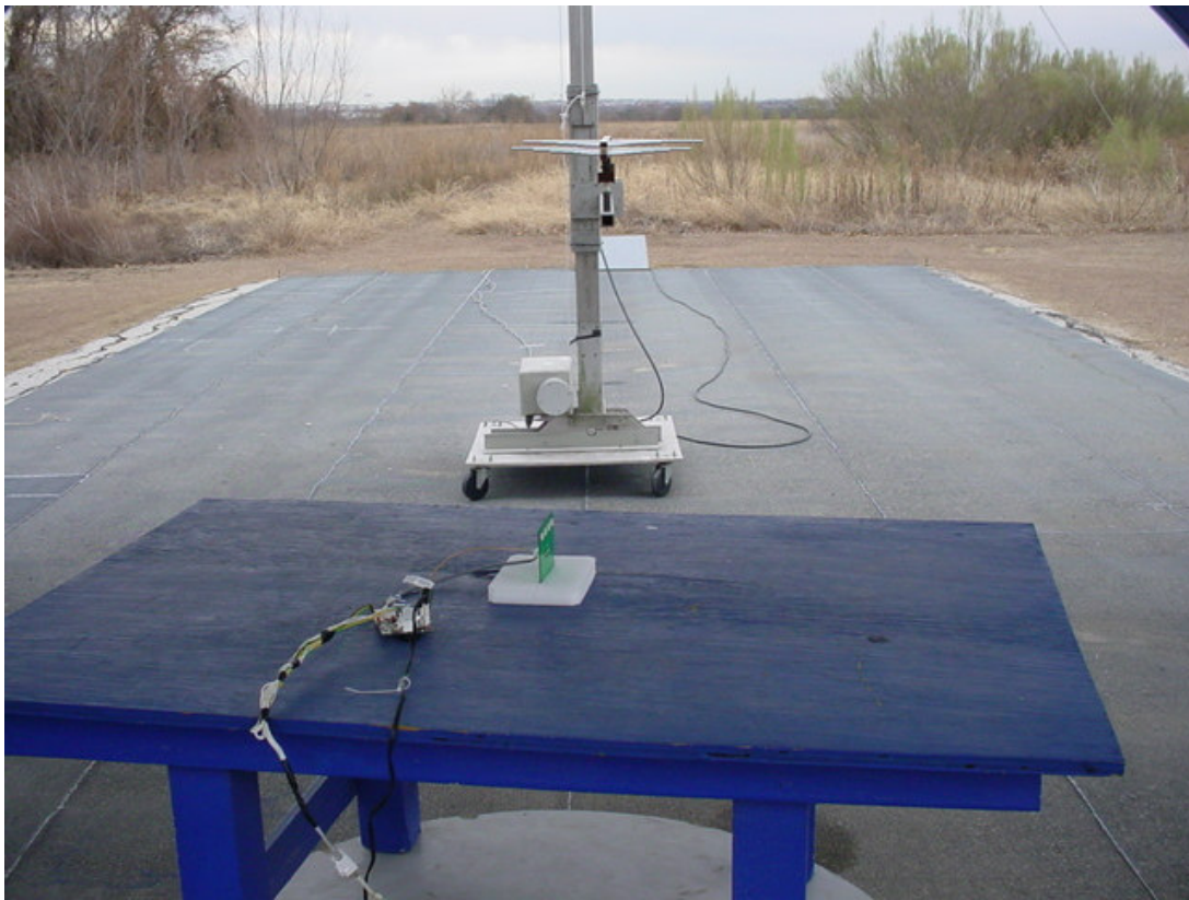
Spurious Emissions
