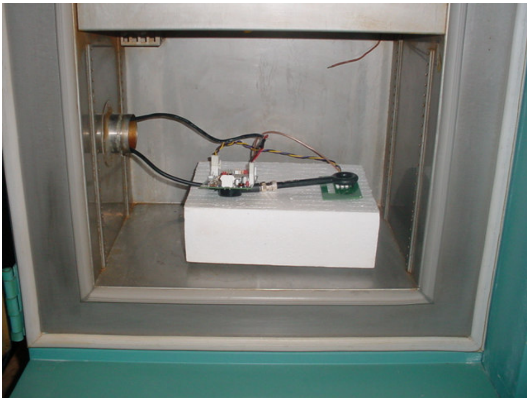
Temperature / Voltage Frequency Stability
