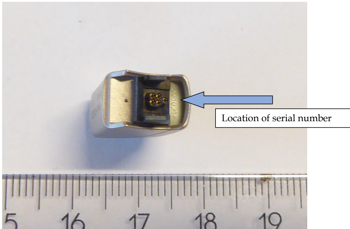
R12G2 adapter (Oticon CS44+1) connector view
