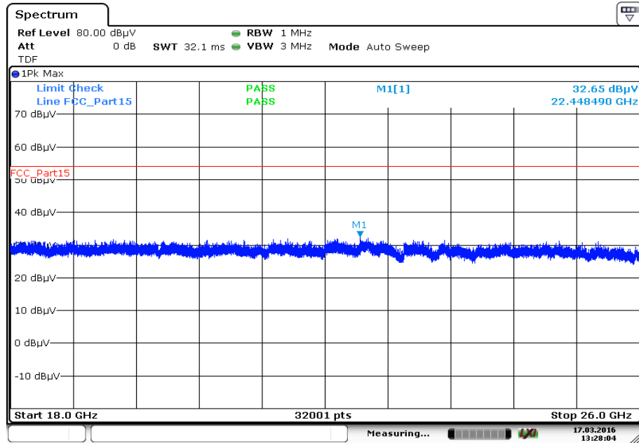
Plot 9: 18 GHz to 26 GHz, TX mode, channel 39, vertical & horizontal polarization, antenna L5
