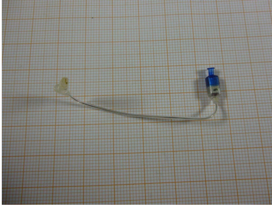
Photo 3: Wire antenna
