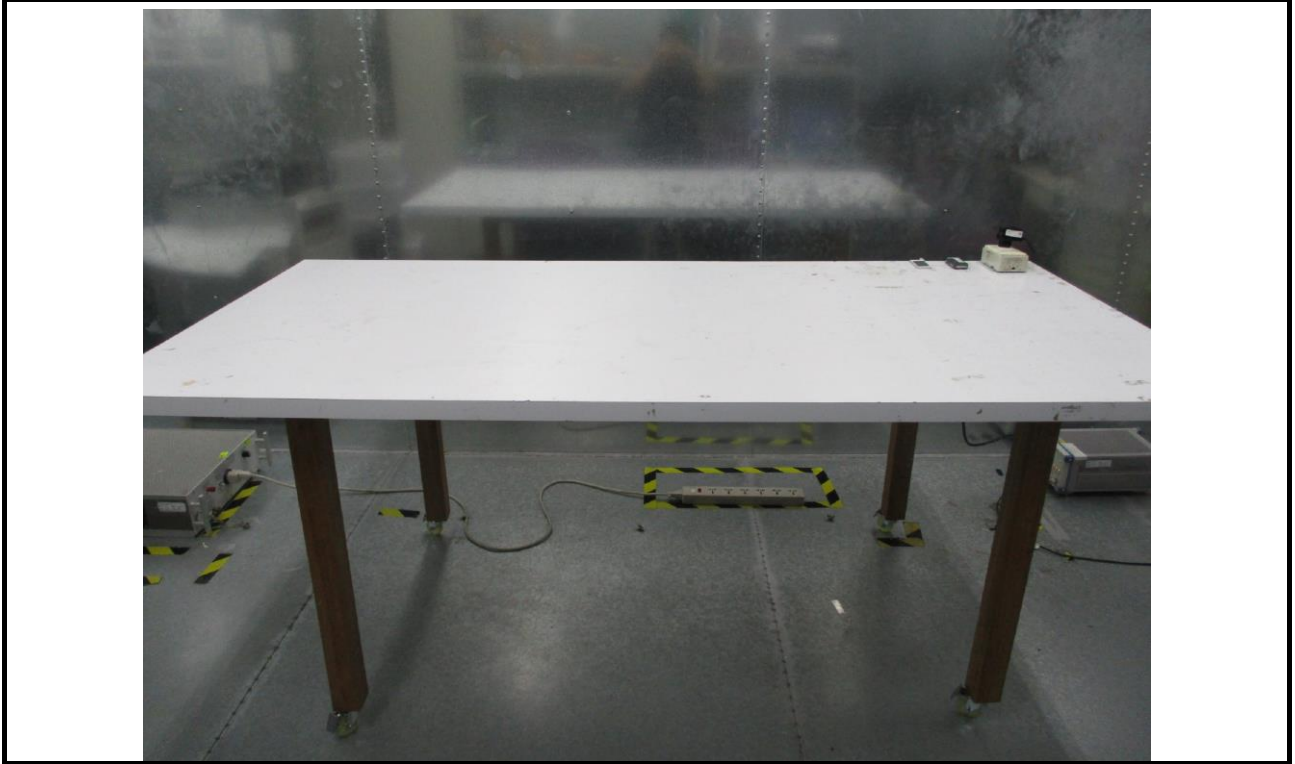
Conducted Emission Test (Ferrite coil antenna, Adapter mode)
