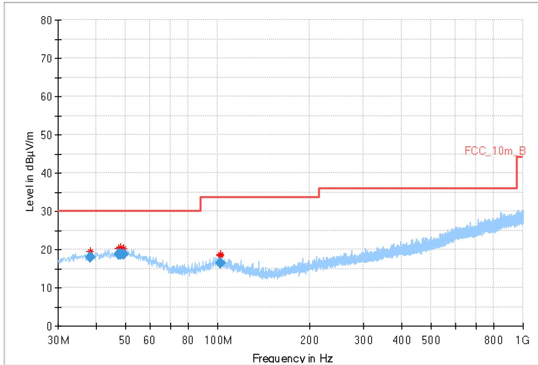
Plot 2: 30 MHz to 1 GHz, TX mode, 2440 MHz, vertical & horizontal polarization, 1 Msp/s
