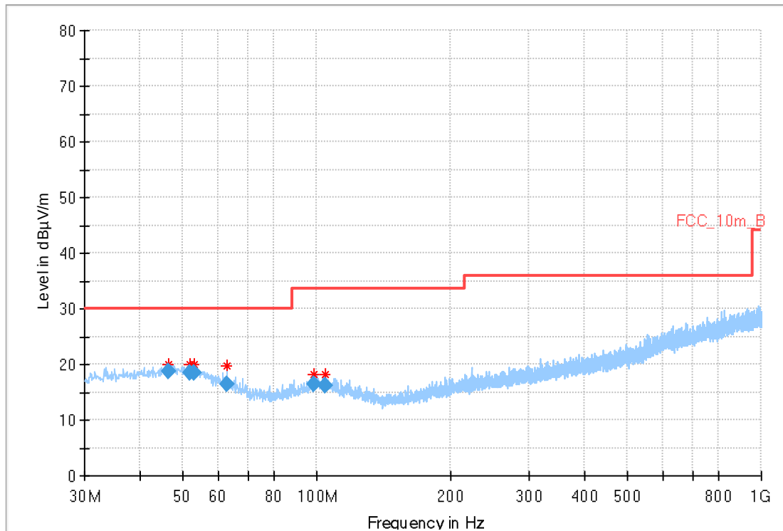
Plot 3: 30 MHz to 1 GHz, TX mode, 2480 MHz, vertical & horizontal polarization, 1 Msps
