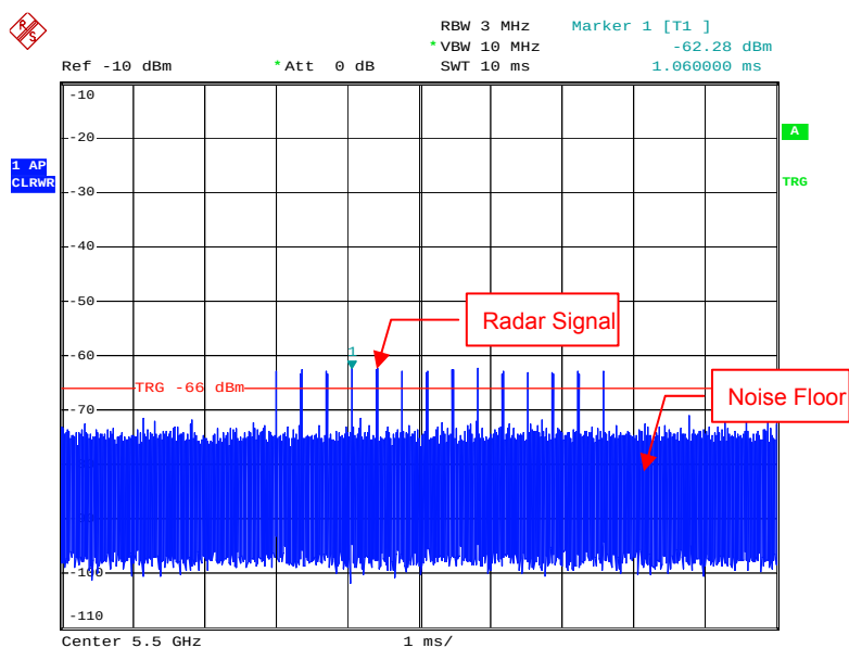
Radar Signal 4
