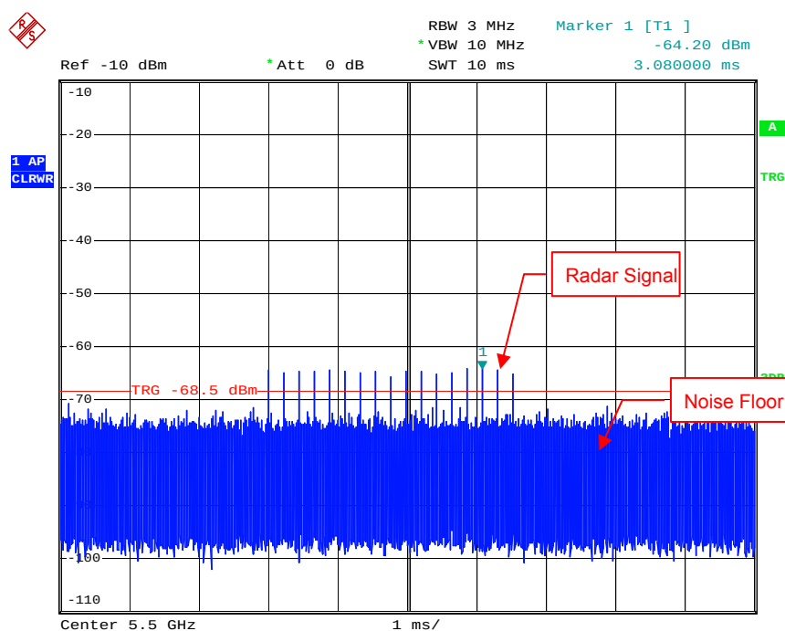
Radar Signal 3
