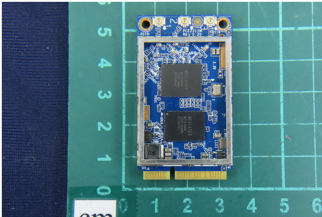
(2) EUT Photo - Model No.: PCE2311M
