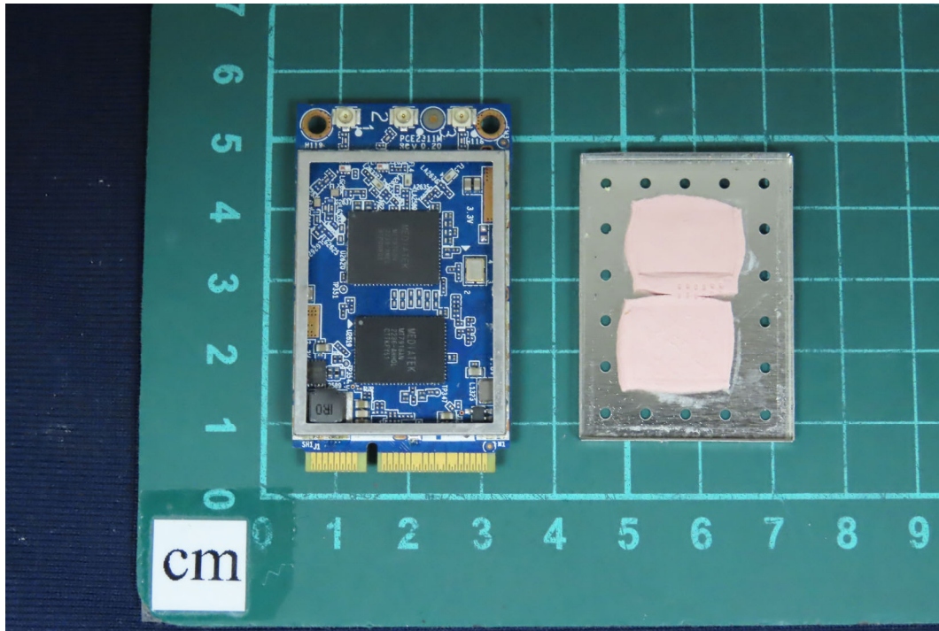
(1) EUT Photo - Model No.: PCE2311M
