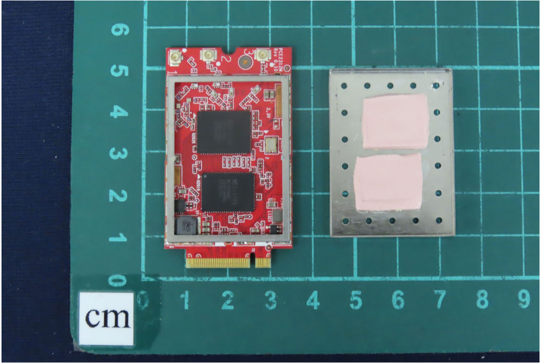
(6) EUT Photo - Model No.: PCE2312M
