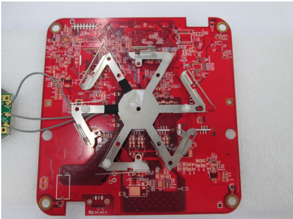
Conducted Test_Ant 3
