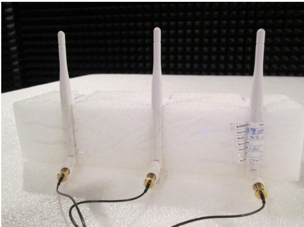
Radiated Test_Ant 1
