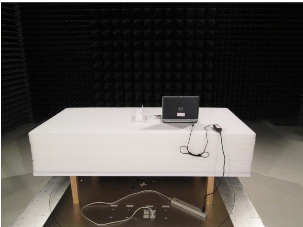
Radiated Test_Ant 1
