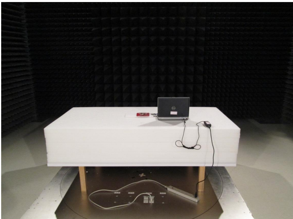
Radiated Test_Ant 3
