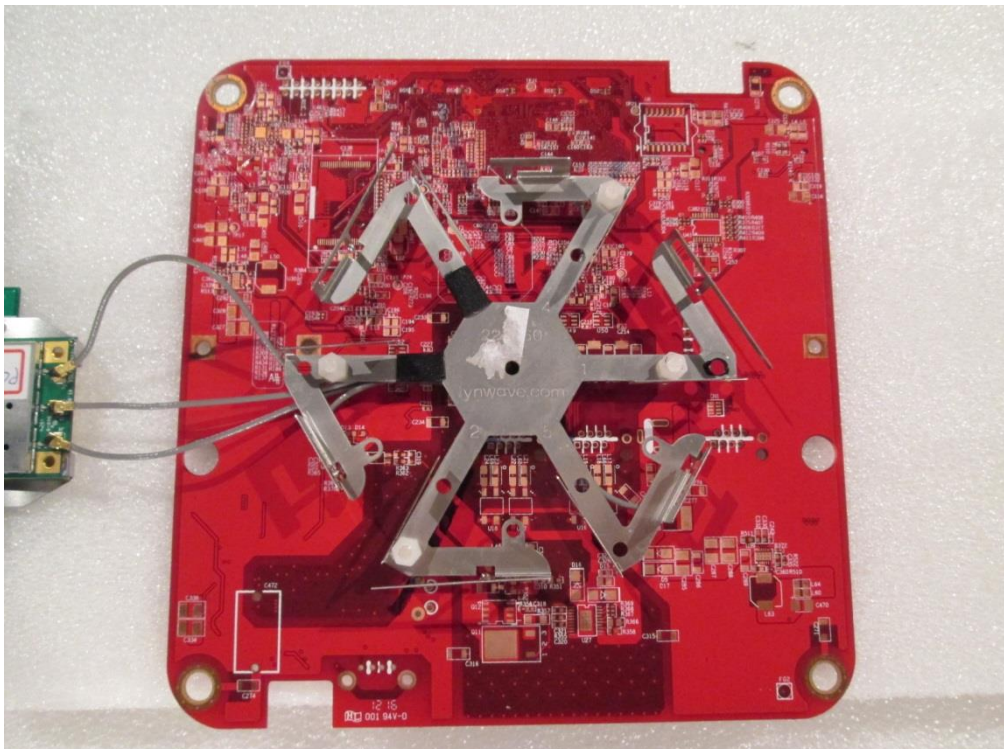
Radiated Test_Ant 3
