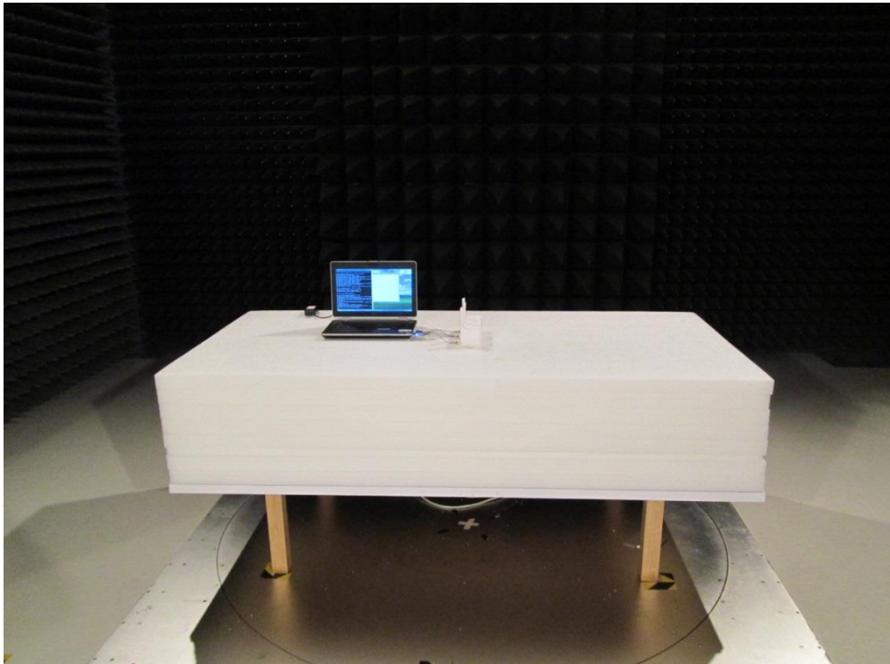
Radiated Test_Ant 2
