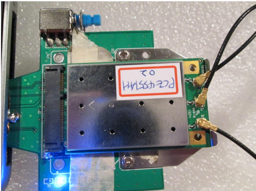
Radiated Test_Ant 2
