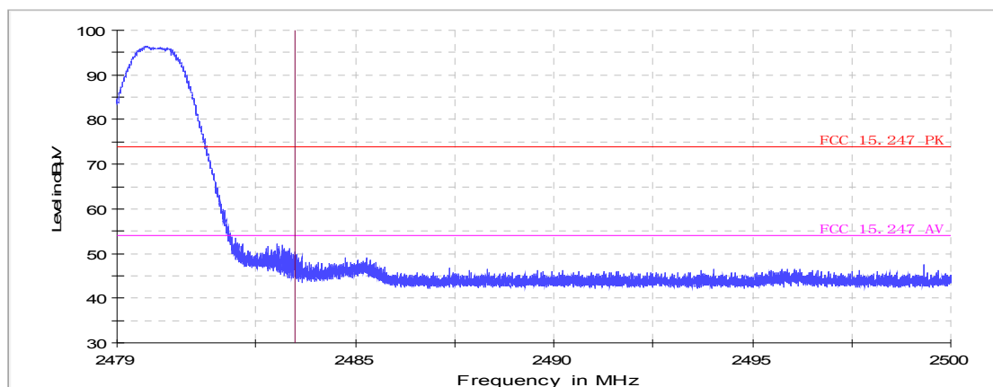
FCC Electric Field Strength 2.4GHz Bandedge-PK
