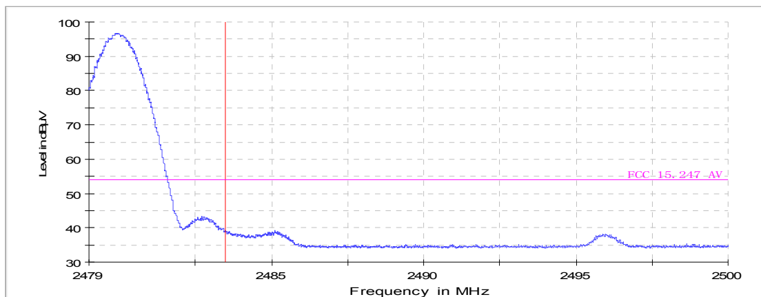
FCC Electric Field Strength 2.4GHz Bandedge-AV
