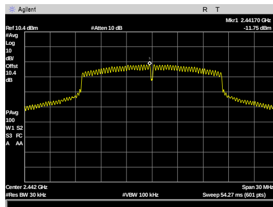
Figure 132: Power Spectral Density, G mode 20M Bw, AVGPSD-2 mid channel
