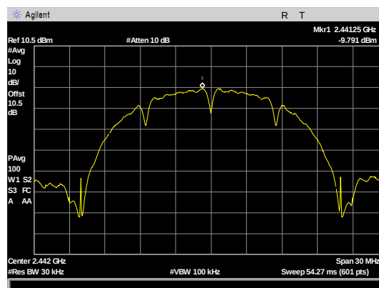
Figure 129: Power Spectral Density, B mode 20M Bw, AVGPSD-2 mid channel
