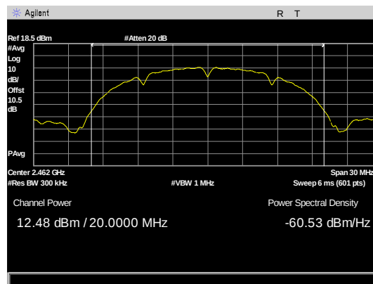
Figure 17: Output Power, B mode 20M Bw AVGSA-2 high channel
