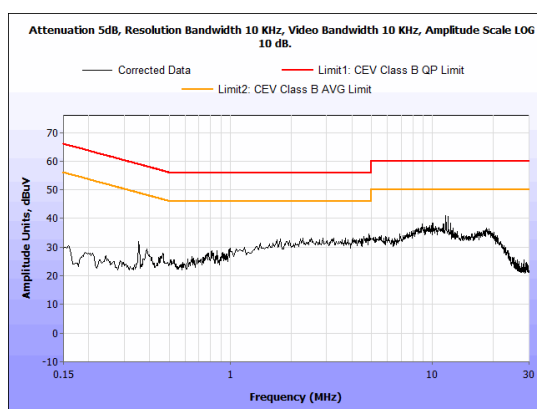
Figure 2. Conducted Emissions, 15.207(a), Phase Line
