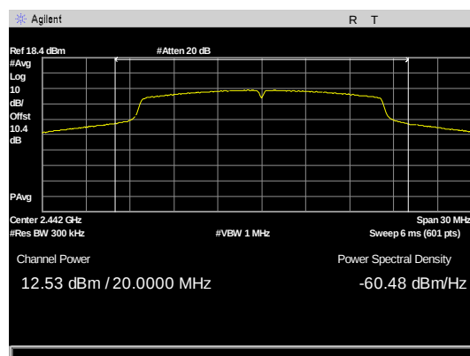
Figure 22: Output Power, G mode 20M Bw AVGSA-2 mid channel
