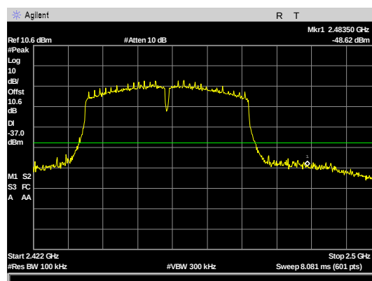
Figure 127: Conducted Spurious Emissions, N mode 40M Bw, AVGSA-2 high channel bandedge
