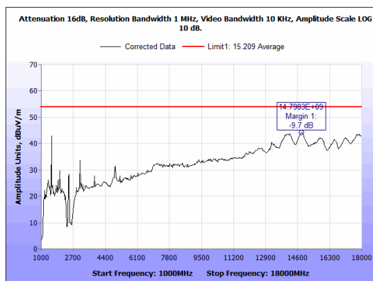
Figure 47: Radiated Spurious Emissions, G mode 20M high channel RE 1-18GHz Average.
