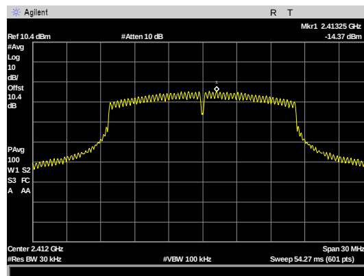
Figure 131: Power Spectral Density, G mode 20M Bw, AVGPSD-2 low channel
