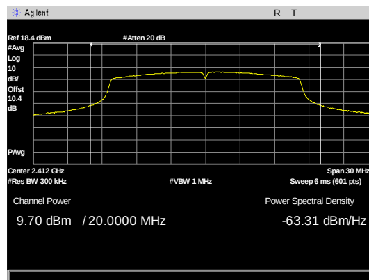
Figure 21: Output Power, G mode 20M Bw AVGSA-2 low channel
