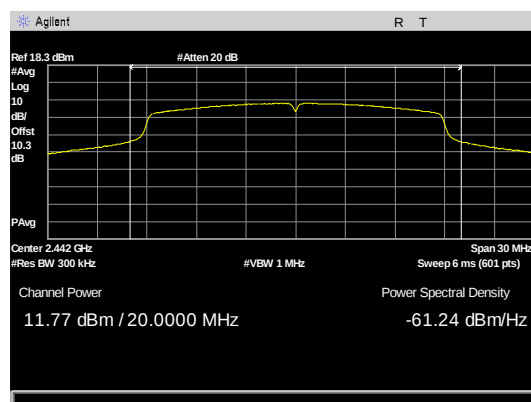
Figure 25: Output Power, N mode 20M Bw AVGSA-2 mid channel
