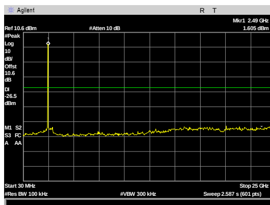
Figure 103: Conducted Spurious Emissions, B mode 20M Bw 30MHz-25GHz, AVGSA-2 high channel
