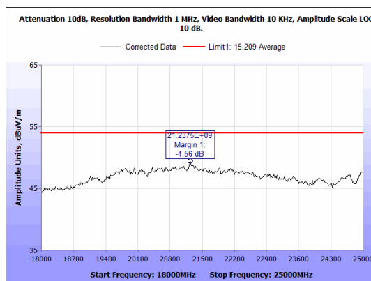
Figure 39: Radiated Spurious Emissions, B mode 20M low channel RE 18-25GHz Average.
