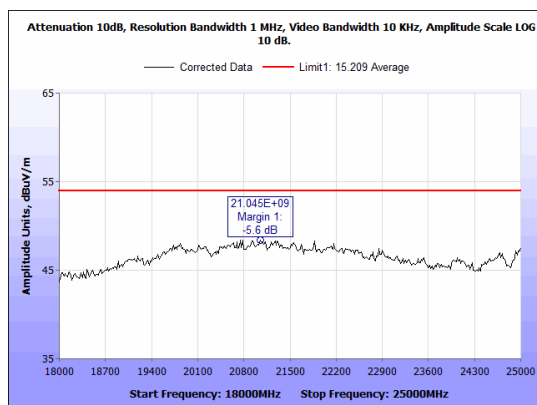
Figure 48: Radiated Spurious Emissions, G mode 20M high channel RE 18-25GHz Average.
