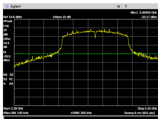
Figure 124. Conducted Spurious Emissions, N Mode 20M Bw, AVGSA-2 low Channel Bandedge
