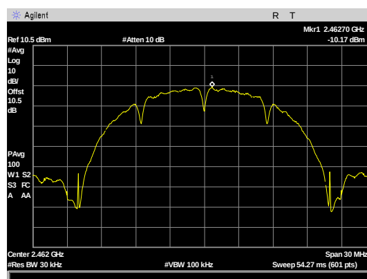
Figure 130: Power Spectral Density, B mode 20M Bw, AVGPSD-2 high channel
