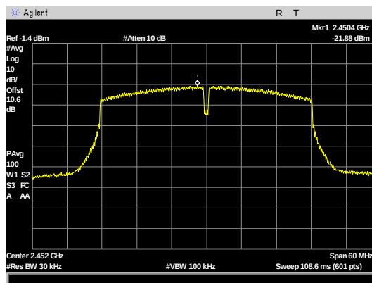
Figure 138: Power Spectral Density, N mode 40M Bw, AVGPSD-2 high channel
