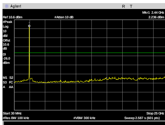
Figure 101: Conducted Spurious Emissions, B mode 20M Bw 30MHz-25GHz, AVGSA-2 mid channel
