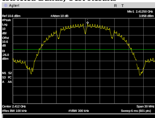
Figure 98: Conducted Spurious Emissions, B mode 20M Bw, AVGSA-2 low channel Reference Level
