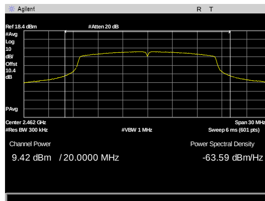
Figure 20: Output Power, G mode 20M Bw AVGSA-2 high channel
