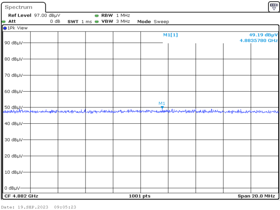
F2 X2 4882.0 Harmonic Vertical PEAK
