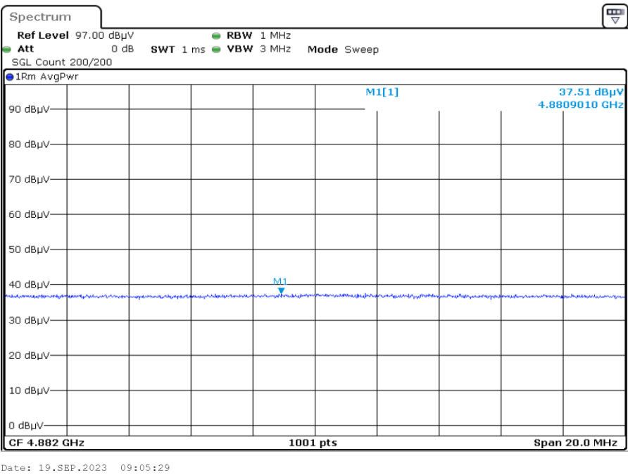
F2 X2 4882.0 Harmonic Vertical AVG
