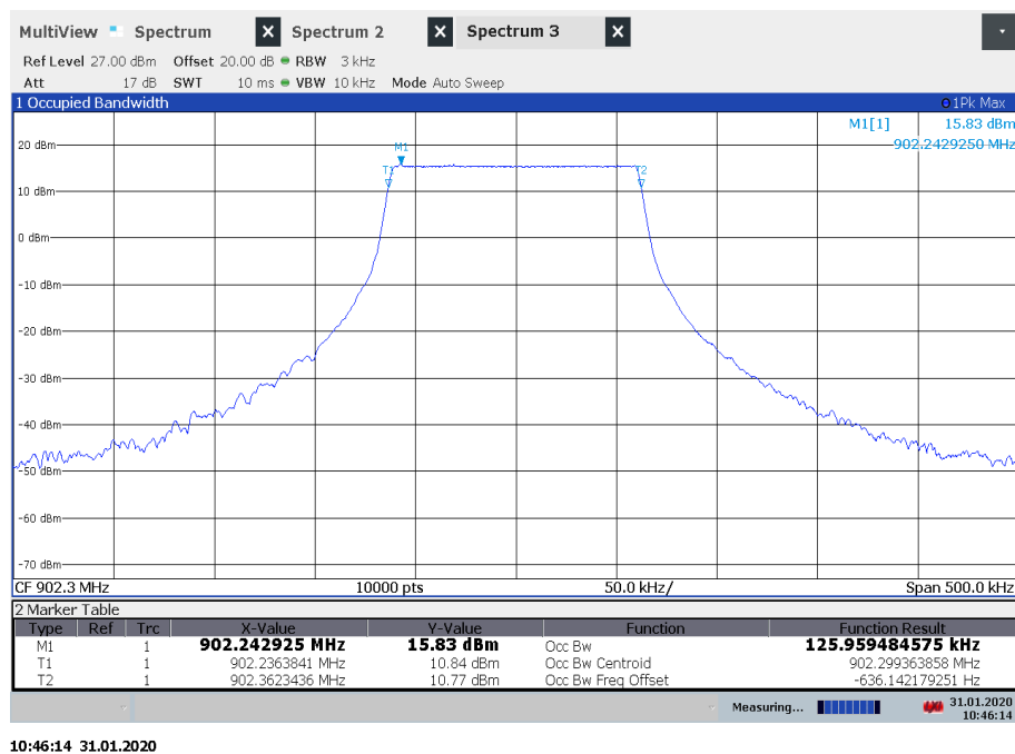
Plot 2: Lowest Channel, 99%OBW
