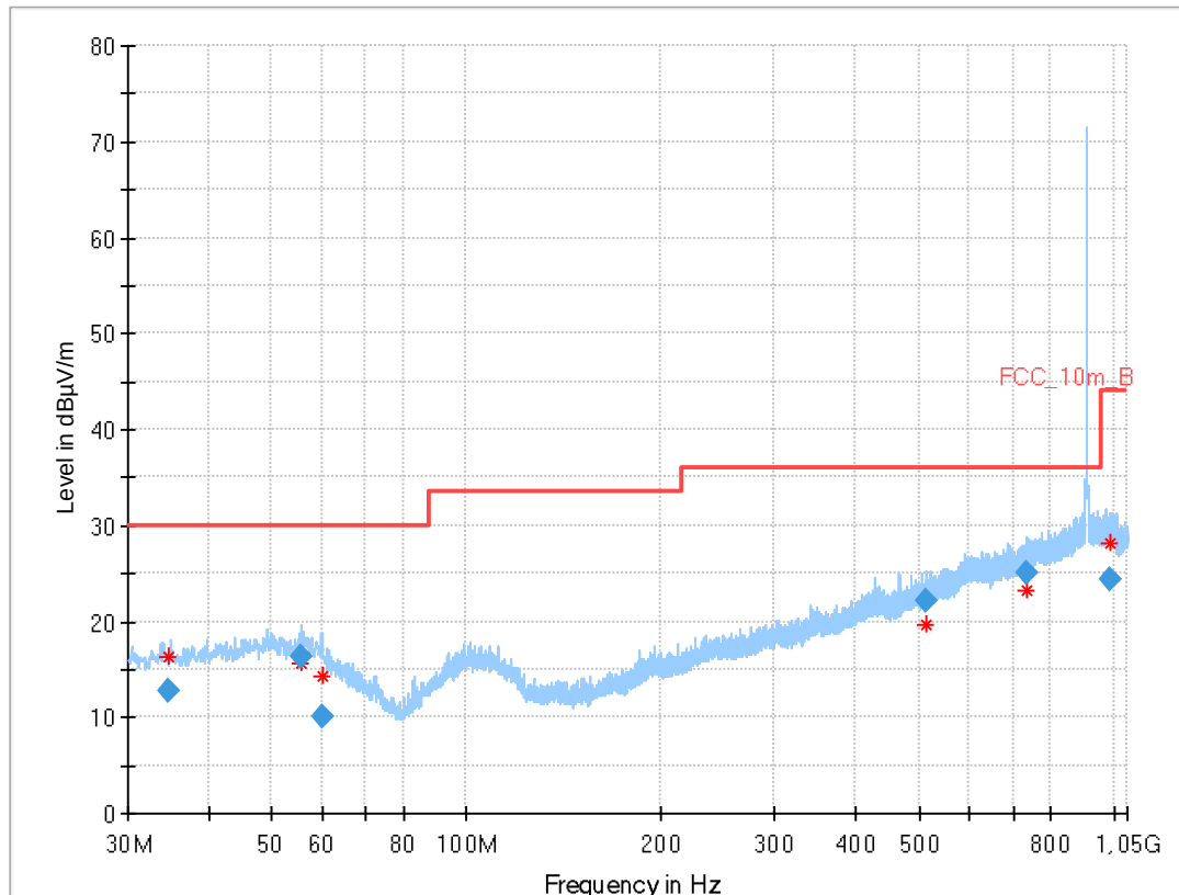
Plot 2: 30 MHz – 1 GHz, horizontal &amp; vertical polarisation (middle channel)
