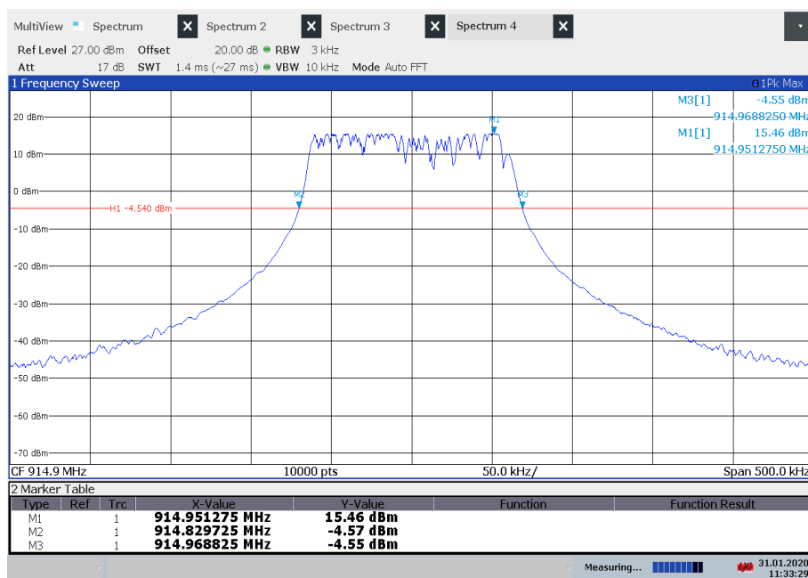
Plot 3: Highest Channel, 20 dB-BW
