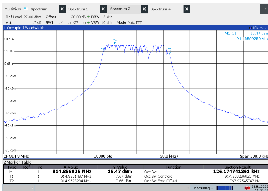
Plot 2: Highest Channel, 99%OBW
