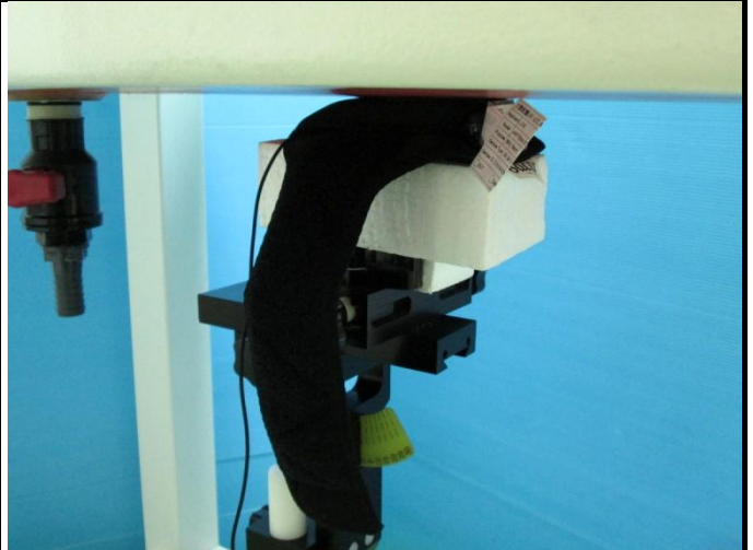
Rear Face of EUT with 0 cm Gap with Holster 1
