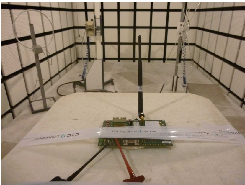
Photo 4: EUT at the anechoic chamber, dipole antenna
