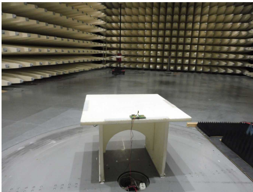
Photo 12: EUT at the semi-anechoic chamber, PCB antenna
