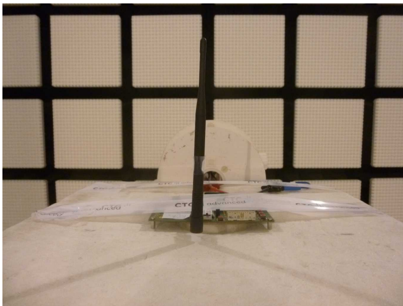
Photo 2: EUT at the anechoic chamber, dipole antenna
