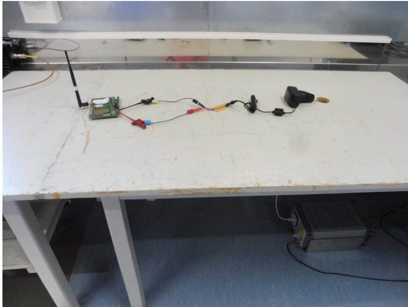
Photo 13: AC conducted emission test setup with dipole antenna
