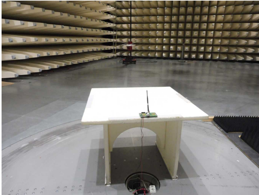
Photo 11: EUT at the semi-anechoic chamber, dipole antenna
