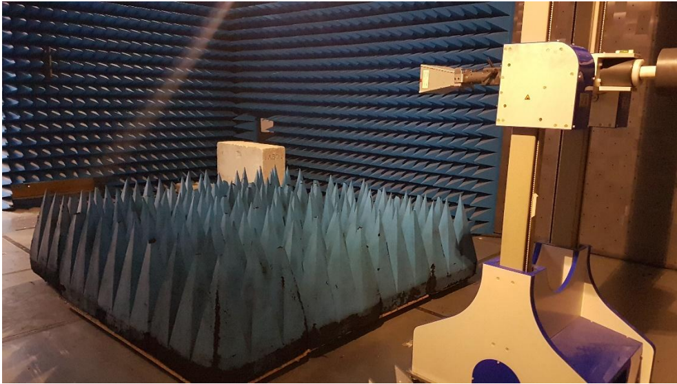
Radiated measurement setup above 1 GHz
