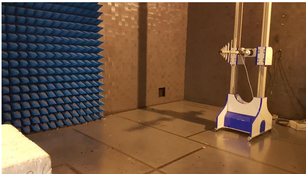
Radiated measurement setup between 200 MHz to 1000 MHz
