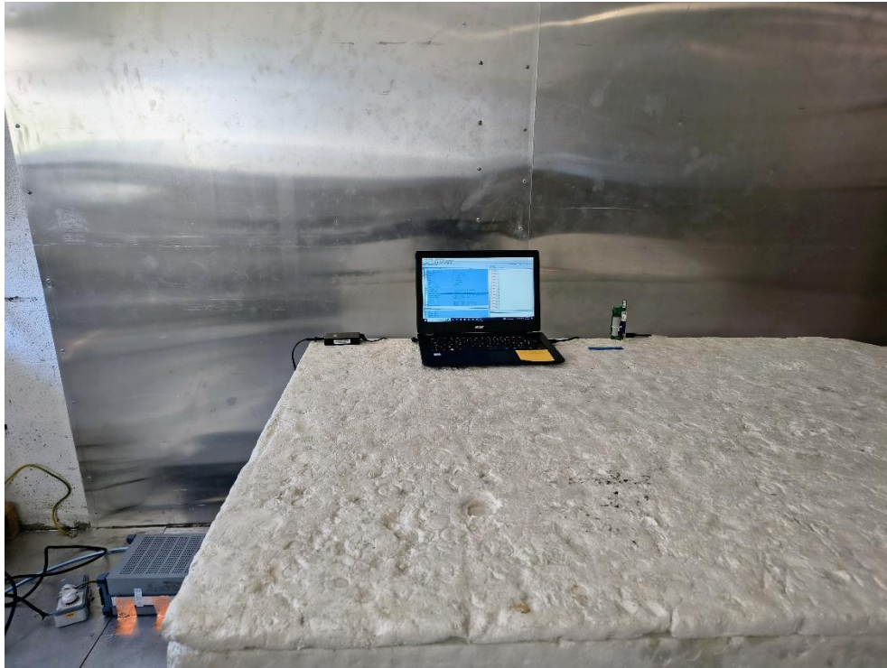
Conducted measurement setup
