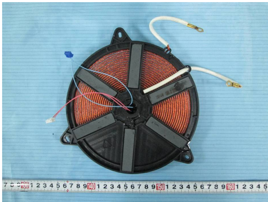
EUT – Coil Rear View
