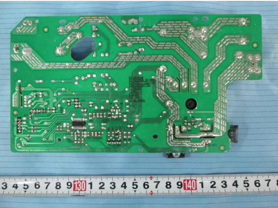
EUT –Main Board Shielding-off Rear View
