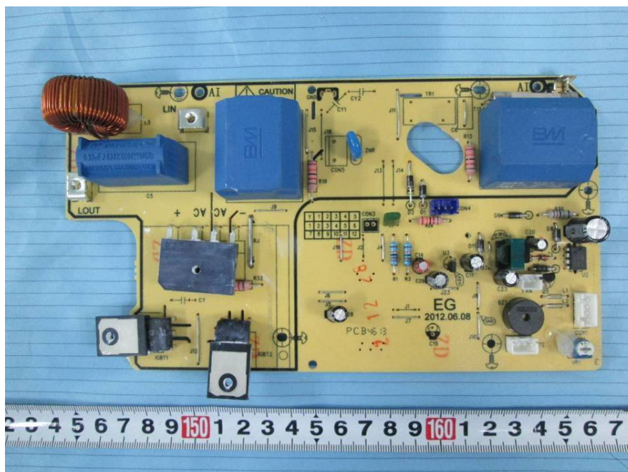
EUT –Main Board Shielding-off Front View
