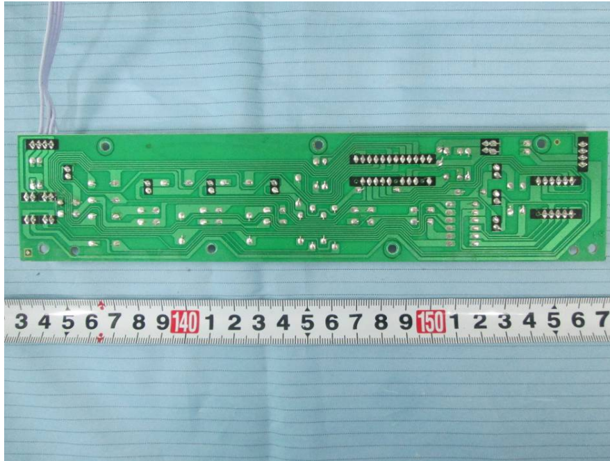
EUT – Right Main Board 1 Bottom View
