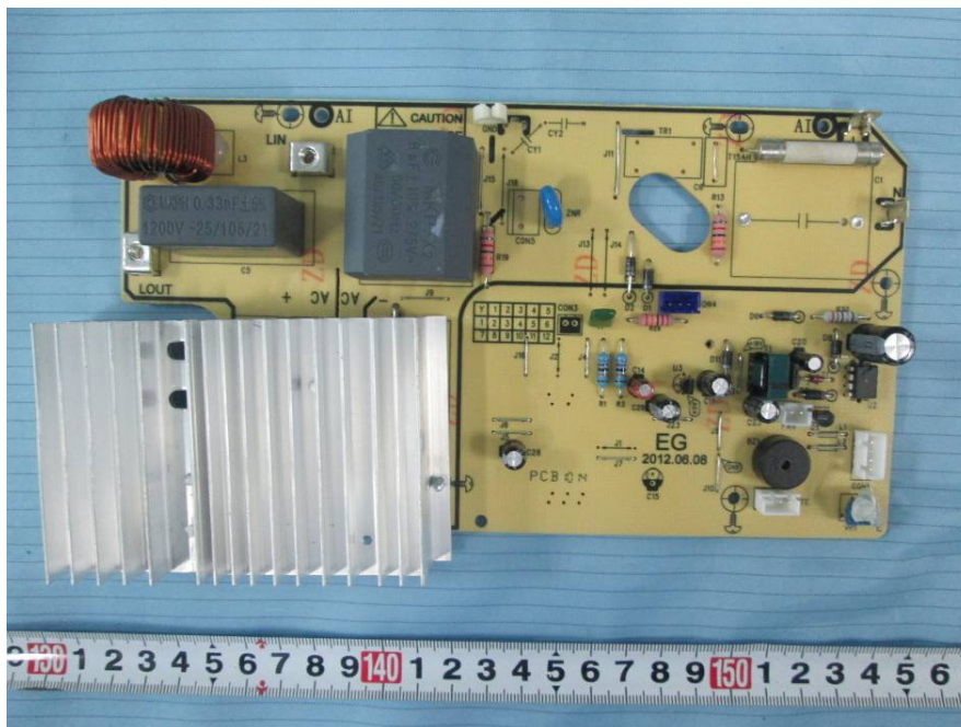
EUT – Cover Right Main Board 3 Top View
