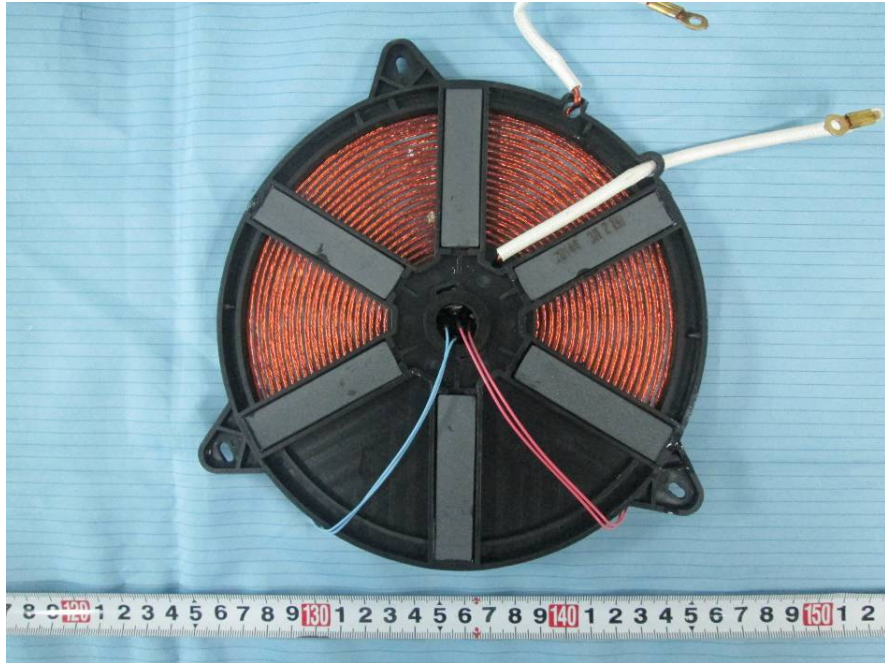
EUT – Left Coil Bottom View
