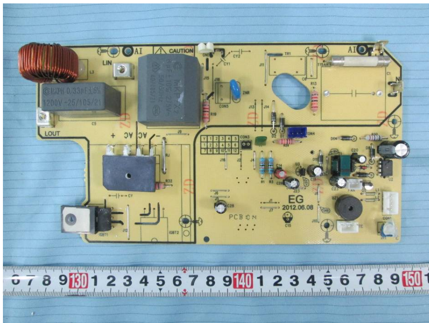
EUT – Uncovered Right Main Board 3 Top View
