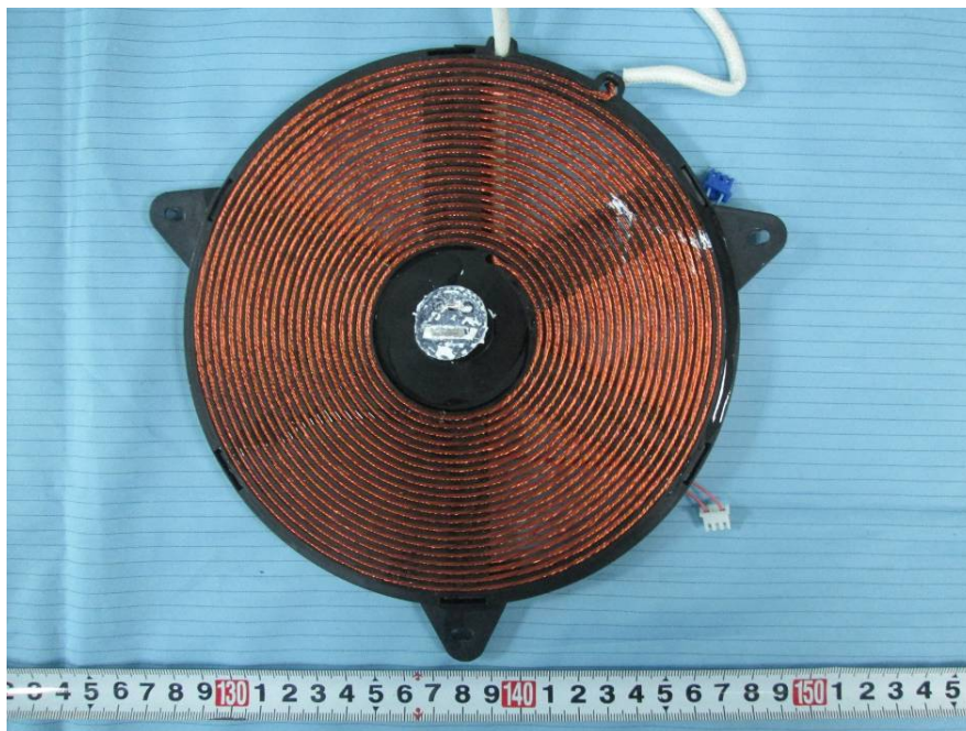
EUT – Left Coil Top View
