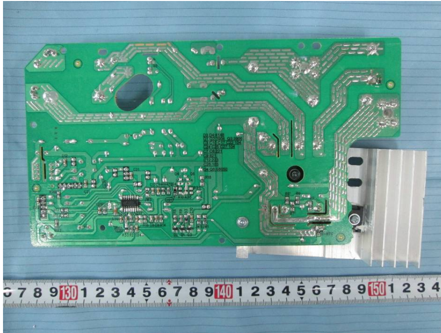
EUT – Cover Left Main Board 3 Bottom View
