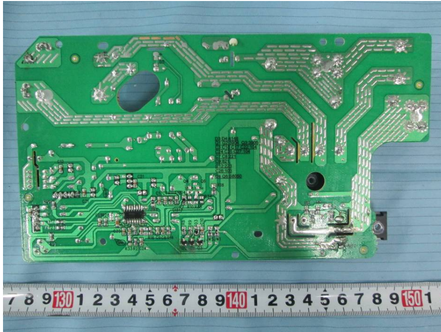
EUT – Uncovered Right Main Board 3 Bottom View
