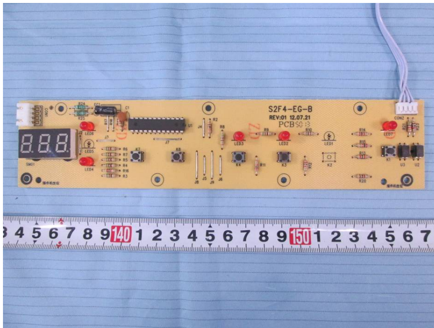
EUT – Right Main Board 1 Top View
