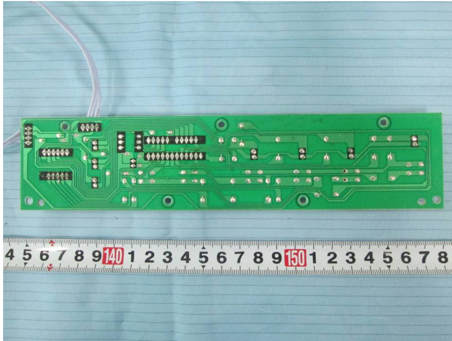
EUT – Left Main Board 1 Bottom View
