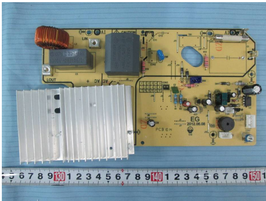
EUT – Cover Left Main Board 3 Top View
