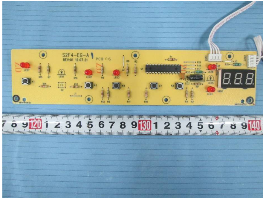
EUT – Control Board 2 Top View
