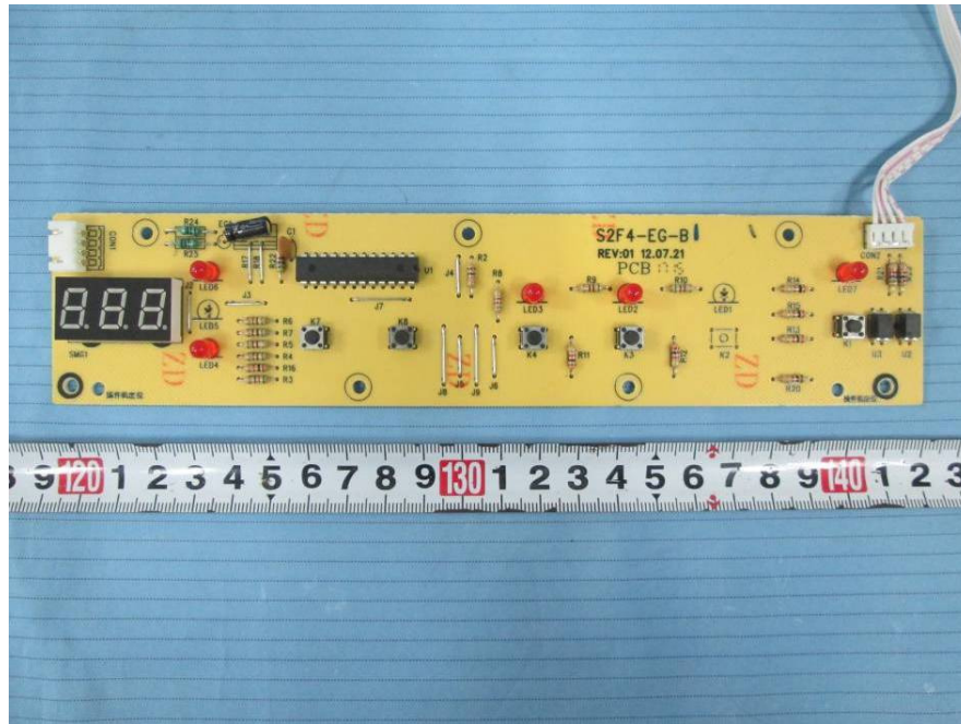
EUT – Control Board 1 Top View
