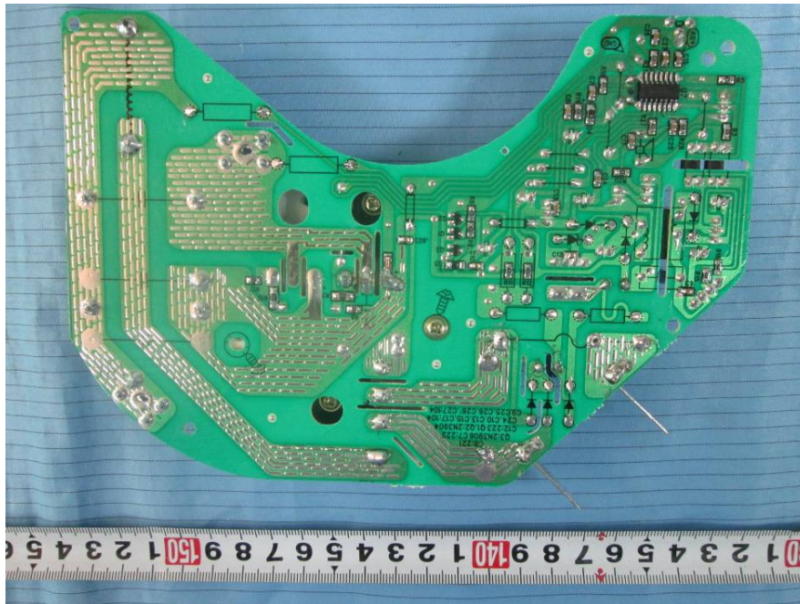
EUT – Left Main Board Bottom View
