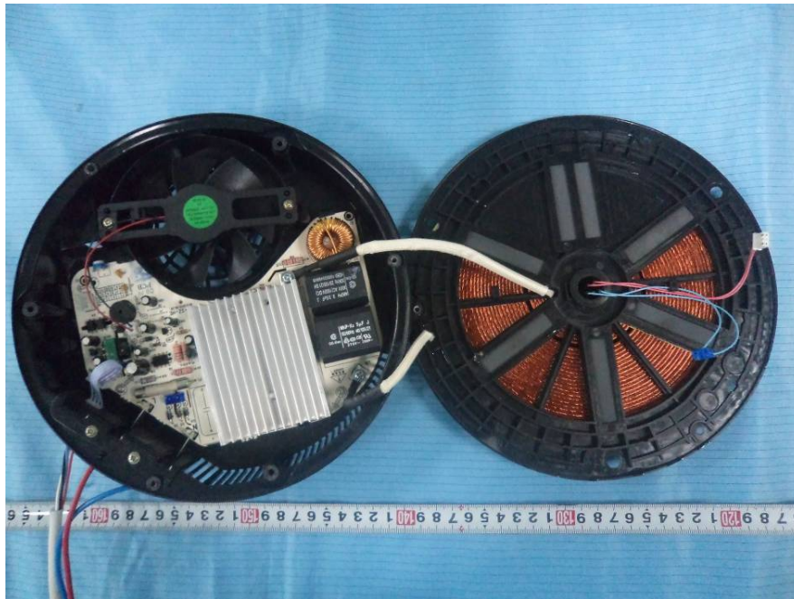
EUT – Left Cover off 2 View
