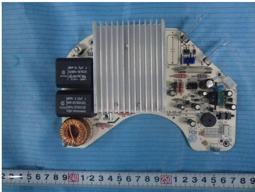
EUT – Left Main Board Top View
