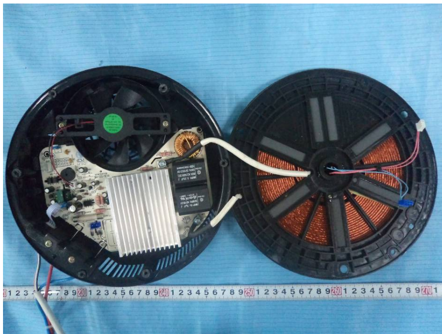
EUT – Right Cover off 2 View
