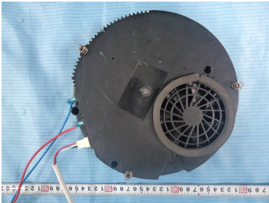
EUT – Left Cover off 1 Back View
