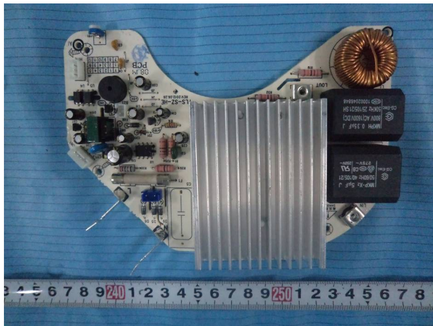
EUT – Right Main Board Top View
