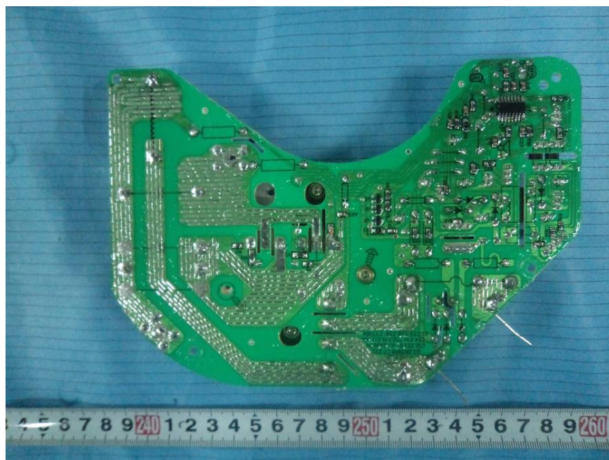
EUT – Right Main Board Bottom View
