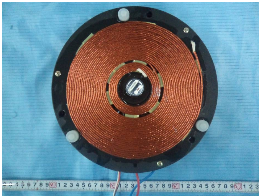
EUT – Right Cover off 1 Front View
