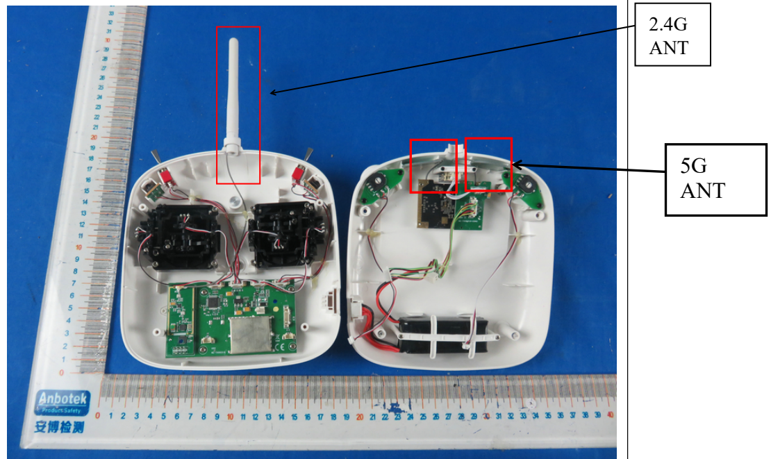
2. Figure PCB of the EUT-Front View
